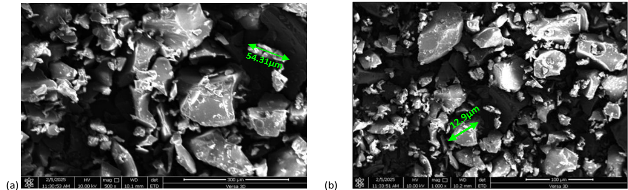
Fig. 1 Surface morphology and particle distribution at (a) 500x magnification and (b) 1000x magnification
