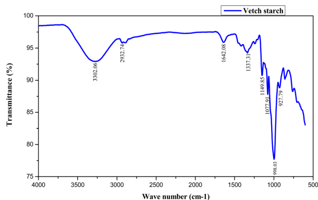
Fig. 1 FTIR spectra of vetch starch.
