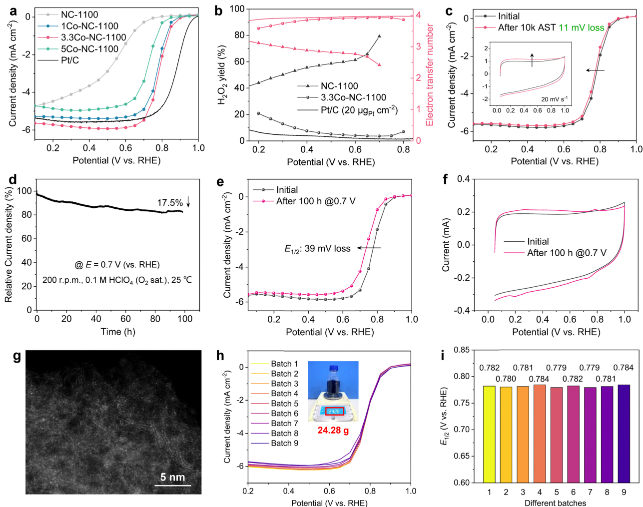
Fig. 4 Electrochemical characterization (in 0.1 M \text{HClO}_4 solution) of the synthesized Co-N-C catalysts. (a) Steady-state ORR polarization plots. (b) ORR selectivity (evaluated by the \text{H}_2\text{O}_2 yield and electron transform number) of the NC-1100, 3.3Co-NC-1100, and Pt/C catalysts. (c) Steady-state ORR polarization plots of the 3.3Co-NC-1100 catalyst before and after square potential cycling ( \text{O}_2 -saturated) between 0.6 and 1.0 V (holding 3 s at each potential). The inset shows the corresponding CV curves before and after the AST. (d) Chronoamperometric curve (@0.7 V) of the 3.3Co-NC-1100 catalyst. (e) Steady-state ORR polarization plots and (f) CV curves before and after the constant-potential test at 0.7 V for 100 h. (g) Aberration-corrected HAADF-STEM images of the 100 h AST-treated 3.3Co-NC-1100 catalyst. (h) Steady-state polarization curves of the 3.3Co-NC-1100 catalysts from 9 parallel batches, the inset showing the single-batch production (24.28 g) from 100-g 3.3Co-ZIF-8 precursors. (i) The comparison of E_{1/2} values calculated from (h).
