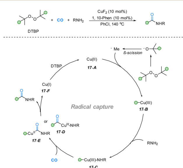
Fig. 17 Radical capture via \beta -scission toward acetamide derivatives.
