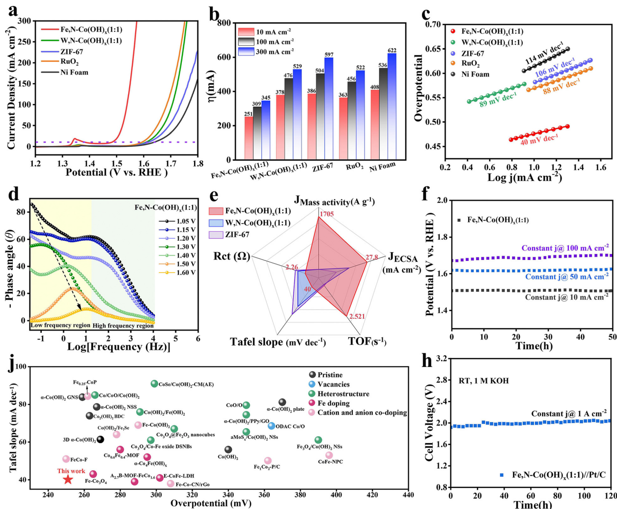
Fig. 3 Electrocatalytic OER activity evaluations. (a) LSV polarization curve in 1 M KOH solution at a scan rate of 5 mV s -1 . (b) Overpotential (η) at 10, 100, and 300 mA cm -2 . (c) Tafel slopes curve. (d) Bode plots for Fe,N-Co(OH) x (1:1) during the OER. (e) Comparison of OER activity between Fe,N-Co(OH) x (1:1) (red), W,N-Co(OH) x (1:1) (blue), and ZIF-67 (orange-red). (f) Chronopotentiometric curve at 10, 50, and 100 mA cm -2 . (g) Comparison with recently reported catalysts. (h) The long-term durability of the prepared AEMWEs (Fe,N-Co(OH) x (1:1)/Pt/C) measured at 1 A cm -2 current density (operated at room temperature at a flow rate of 0.15 L min -1 ).
