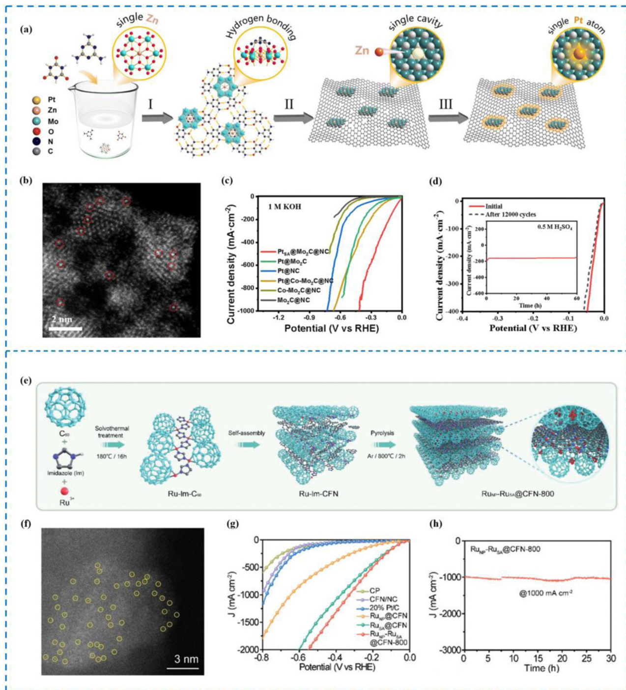
Fig. 9 Synthesis, HAADF-STEM and HER performance of \text{Pt}_{\text{SA}}@Mo_2C@NC (a)–(d) and \text{Ru}_{\text{NP}}-\text{Ru}_{\text{SA}}@CFN-800 (e)–(h). (a) Synthesis of \text{Pt}_{\text{SA}}@Mo_2C@NC . (b) HAADF-STEM image. (c) High current density LSV curve. (d) Stability performance. (e) Synthesis of \text{Ru}_{\text{NP}}-\text{Ru}_{\text{SA}}@CFN-800 . (f) AC-HAADF-STEM image. (g) High current density LSV curve. (h) Stability performance at high current density. 164,165 This figure has been adapted/reproduced from ref. 164 and 165 with permission from The Royal Society of Chemistry and John Wiley and Sons, copyright©2023 Wiley-VCH GmbH.
