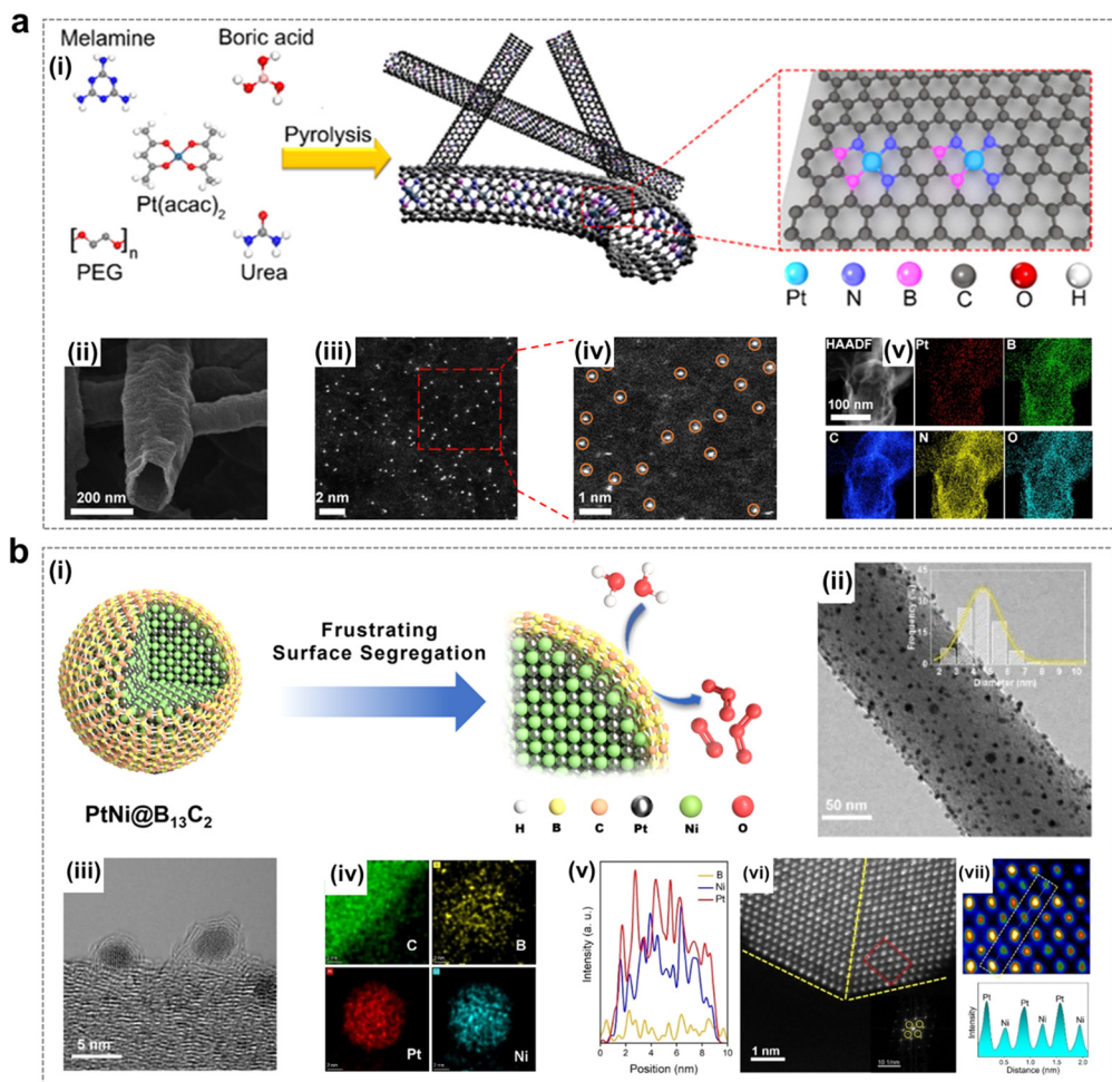
Fig. 8 Pt-containing catalysts using for EOP process. (a) (i) Schematic illustration of the synthesis of Pt-SAs/BNCs. (ii)–(iv) Field-emission SEM, HAADF-STEM, and magnified images of Pt-SAs/BNC-3. (v) Elemental maps of Pt, B, C, N, and O for Pt-SAs/BNC-3. (Reprinted with permission from ref. 15. Copyright ACS Publications 2021.) (b) (i) Schematic representation of the PtNi@B 13 C 2 structure and the EOP process. (ii) and (iii) TEM images of PtNi@B 13 C 2 -2. (iv) EDX elemental maps of C, B, Pt, and Ni for PtNi@B 13 C 2 -2. (v) EDX elemental line scan across a single PtNi@B 13 C 2 -2 nanoparticle. (vi) Enlarged HAADF-HRSTEM image of PtNi@B 13 C 2 -2. (vii) Enlarged view of the region marked by the yellow dotted rectangle in (vi), along with a profile of the atom columns as indicated in the rectangular area of the HAADF-HRSTEM image. (Reprinted with permission from ref. 50. Copyright ACS Publications 2023.)
