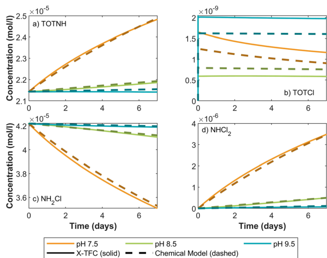
Fig. 4 CKP1 X-TFC results for out-of-sample pH values compared to chemical model using ode15s: a) TOTNH, b) TOTCl, c) NH 2 Cl, and d) NHCl 2 . X-TFC (solid lines), chemical model (dashed lines), different pH values (colored lines).
