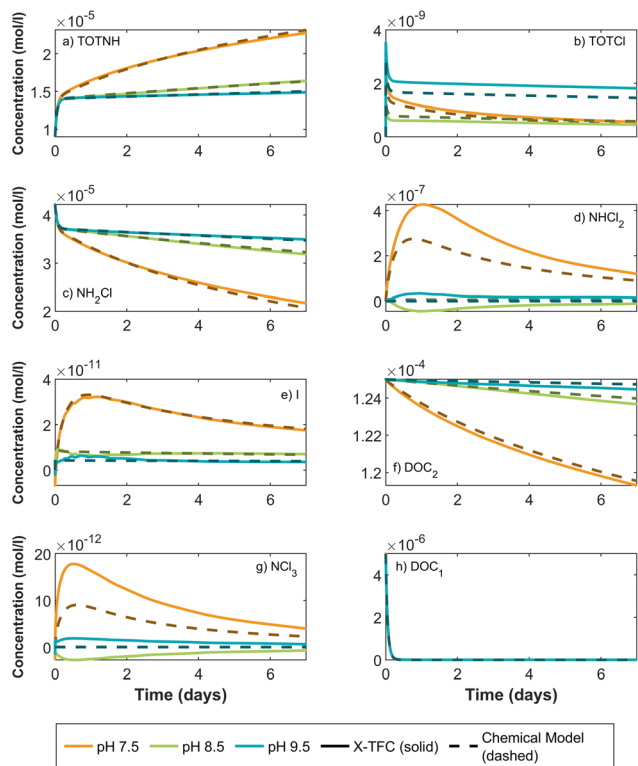
Fig. 5 CKP2 X-TFC results for out-of-sample pH values compared to chemical model solved using ode15s: a) TOTNH, b) TOTCl, c) NH 2 Cl, d) NHCl 2 , e) I, f) DOC 2 , g) NCl 3 , and h) DOC 1 . X-TFC (solid lines), chemical model (dashed lines), different pH values (colored lines). Note that DOC 1 does not vary with pH, hence the lines for different pH values overlap.
