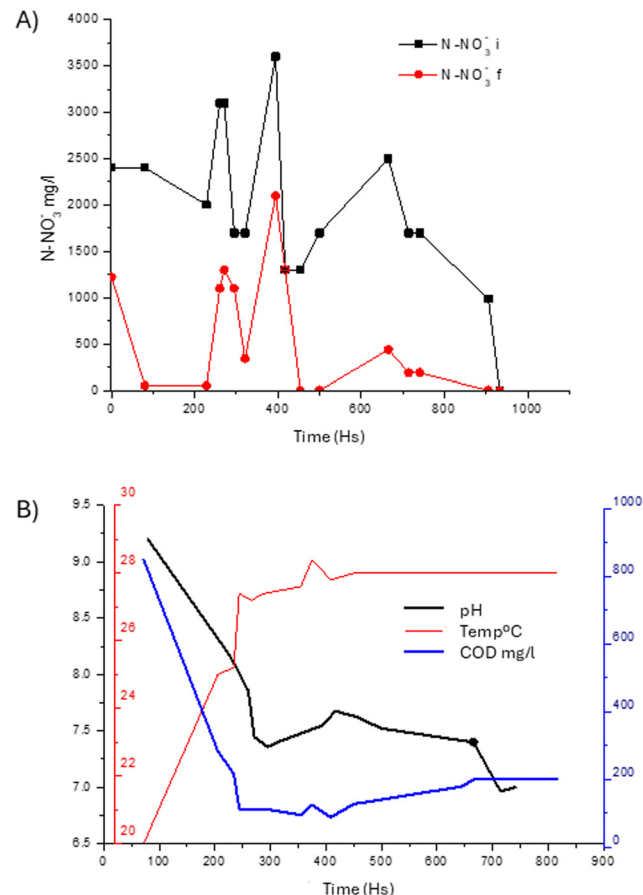
Fig. 6 Denitrification process in FBBRs: A) denitrification performance and B) monitored parameters: pH, T ( ^{\circ}C ), and COD.
