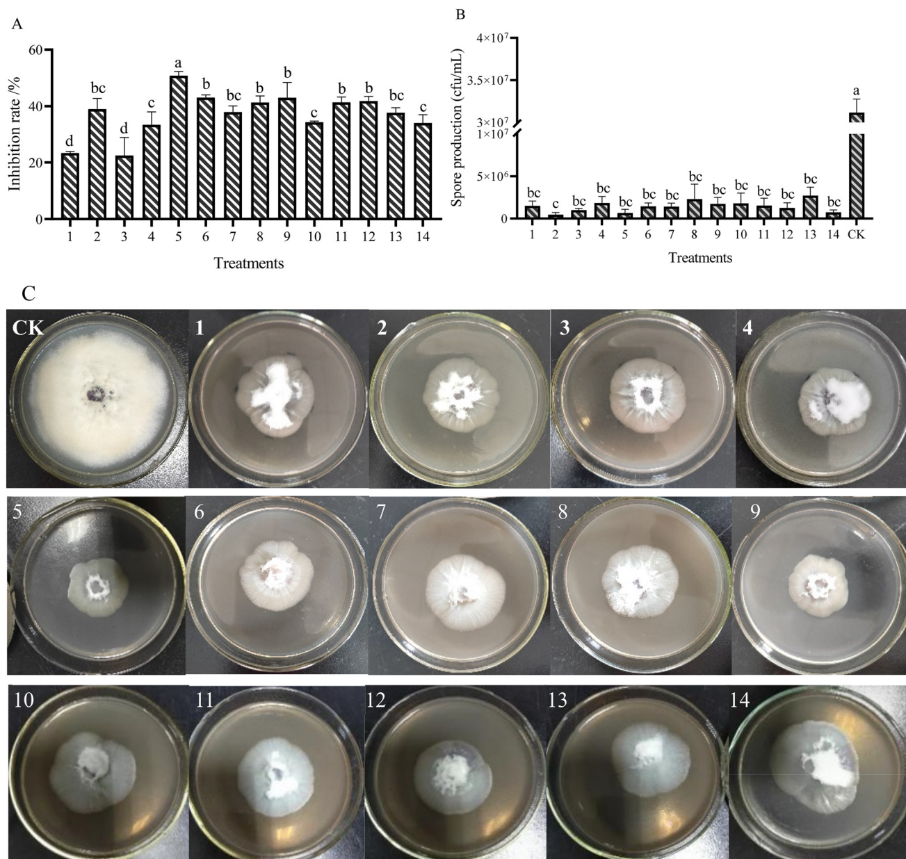
Fig. 2 AgNPs impair the growth and asexual development of F. oxysporum . (A) Inhibition rate of mycelium different. (B) Spore production inhibited by AgNPs. (C) Colony morphology of the FOM cultured on PDA containing different AgNPs for 7 days. 1–14 present the different AgNPs and their combination. 1: AgNPs-TH; 2: AgNPs-TK; 3: AgNPs-TA-FC; 4: AgNPs-TA-XML; 5: 1 + 2; 6: 1 + 3; 7: 1 + 4; 8: 2 + 3; 9: 2 + 4; 10: 3 + 4; 11: 1 + 2 + 3; 12: 1 + 2 + 4; 13: 2 + 3 + 4; 14: 1 + 2 + 3 + 4. Different letter(s) in the same column differ significantly according to Duncan's test ( p < 0.05 ).
