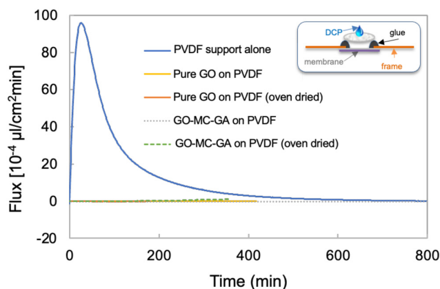
Fig. 6 Diethyl chlorophosphate (DCP) permeation rates through GO (3 μm) and GO-MC-GA (10 μm) films under conditions of vapor-only contact. All films are supported on a porous PVDF filter during testing, which allows rapid DCP vapor permeation when used alone as a positive control. All films studied here are effective DCP vapor barriers.
