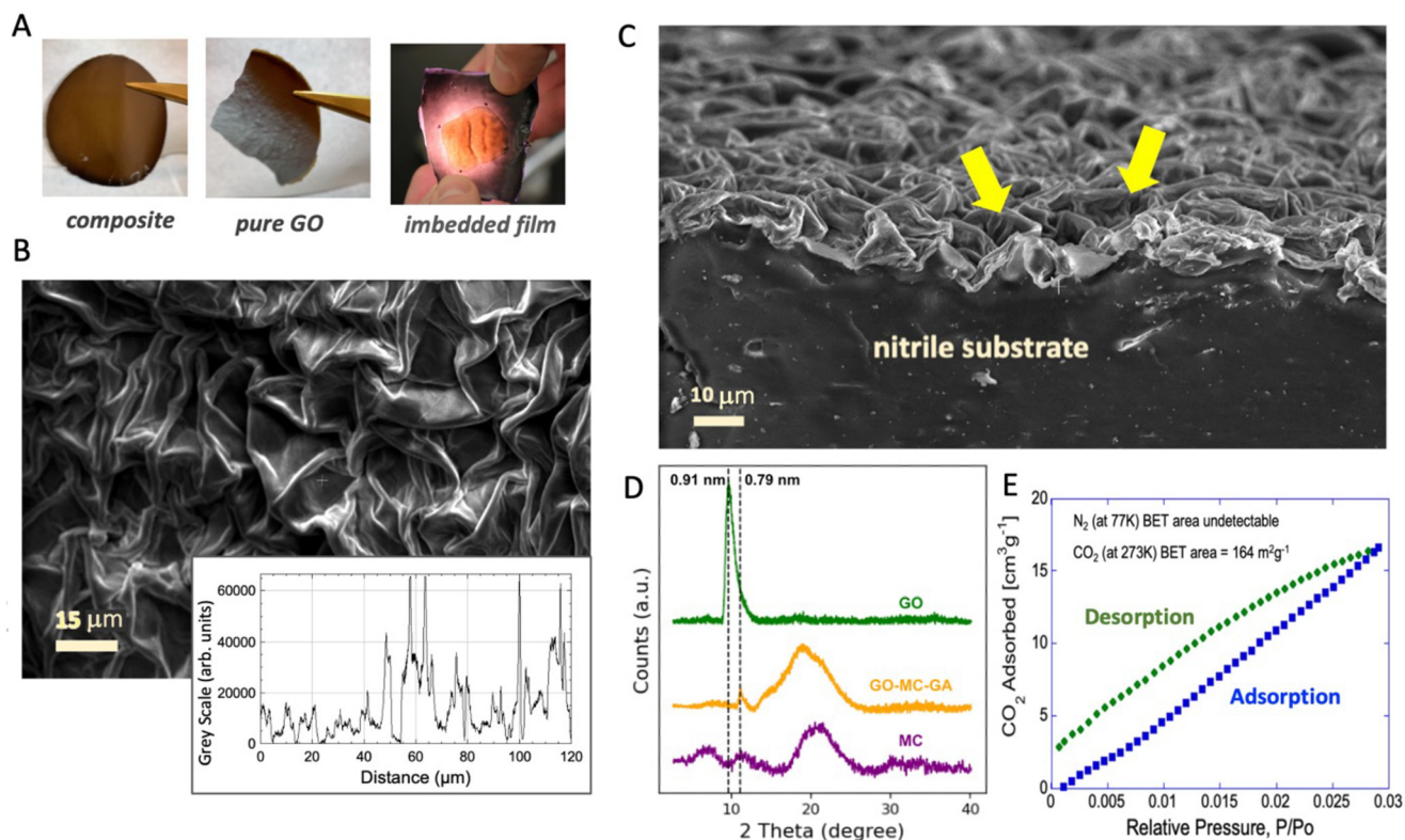
Fig. 3 Structural characterization of graphene-based films. A : Photos of pure, composite and imbedded GO films. The composite films are noticeably less flexible (have higher bending stiffness) than pure GO films. B : Textured GO films fabricated by the mechanical stretch method at 66% isotropic pre-stretch. Inset is a grey-scale line profile showing a \sim 10 \mu\text{m} wavelength scale for the primary out-of-plane textural features. C : Cross-sectional view of a textured GO film (66% pre-stretch) after freeze fracture using tilt-stage SEM (yellow arrows show example complex, 3D cavities). D : XRD spectra for pure GO, the composite, and pure methyl cellulose, showing the interlayer spacing in pure GO films (0.91 nm), and its absence in the GO-MC-GA composite, indicating the loss of nanosheet when the polymer is introduced. E : Vapor adsorption isotherms and computed internal surface areas for the GO-MC-GA film.
