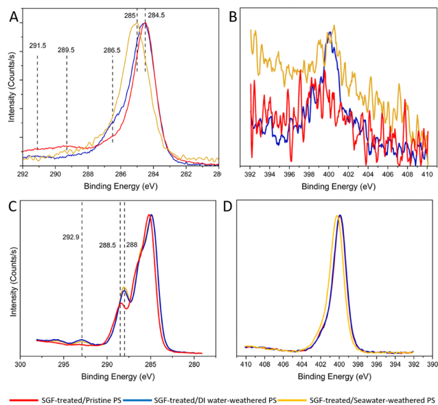
Fig. 3 XPS analysis of particle surface oxidation status and nitrogen composition. A. C1s spectra for pristine PS (red), DI water-weathered PS (blue), seawater-weathered PS (yellow); B. N1s spectra for spectra for pristine, DI water-weathered, and seawater-weathered particles; C. C1s spectra for SGF-treated particles; D. N1s spectra for SGF-treated particles.
