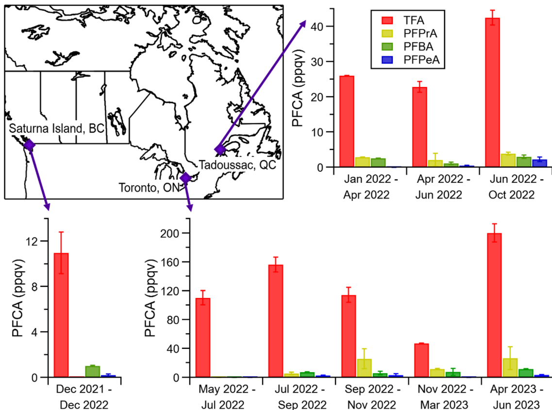
Fig. 3 Measured mean PFCAs mixing ratios (ppqv) for TFA (C2), PFPrA (C3), perfluorobutanoic acid (PFBA, C4), and perfluoropentanoic acid (PFPeA, C5) from three locations in Canada: Saturna Island, BC, Toronto, ON (York University site), and Tadoussac, QC. Error bars show relative error ( n = 2 ) and one standard deviation of replicate ( n \geq 3 ) samples. PFHxA (C6) was not included because of low detection frequency. Mass loadings (units: \text{pg m}^{-3} ) are provided in Table S3,† as these units are used in policy, but not informative in terms of assessing atmospheric formation and fate processes in a consistent manner across the homologue suite of PFCAs.
