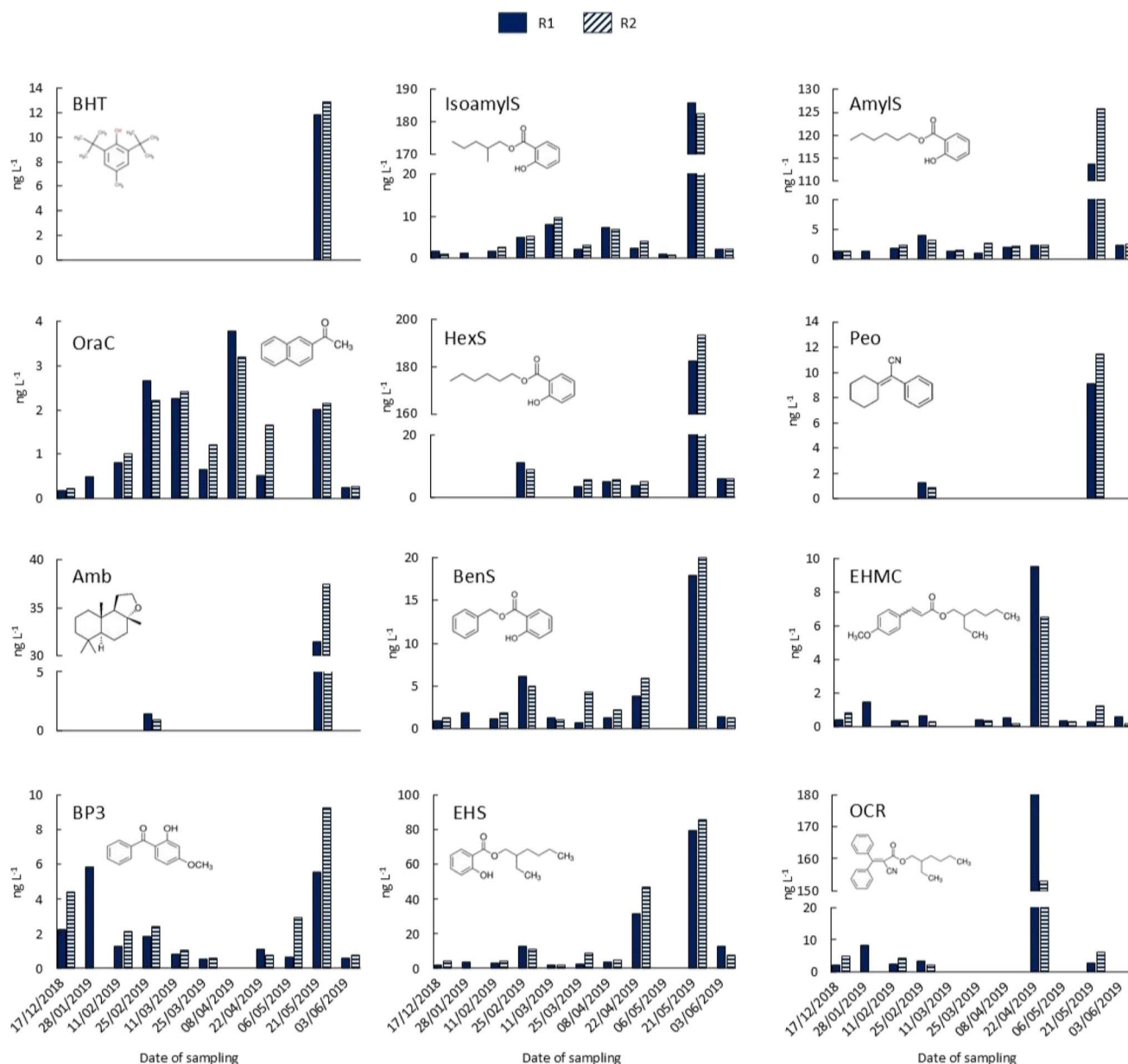
Fig. 2 The concentrations of selected PCP chemicals (ng L -1 ) in the duplicated snow samples (R1 and R2) collected at VRS between mid-December 2018 and the beginning of June 2019.
