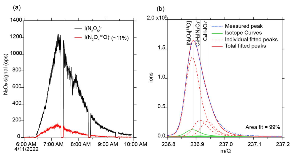
Fig. 7 (a) Adding labeled \text{O}_3 to the house enhanced ^{18}\text{O} - \text{N}_2\text{O}_5 . (b) The I-CIMS separates ^{18}\text{O} -substituted \text{N}_2\text{O}_5 from adjacent ion peaks in the mass spectrum. Note that the timeseries includes periodic zero air measurements; signals decrease during this time.
