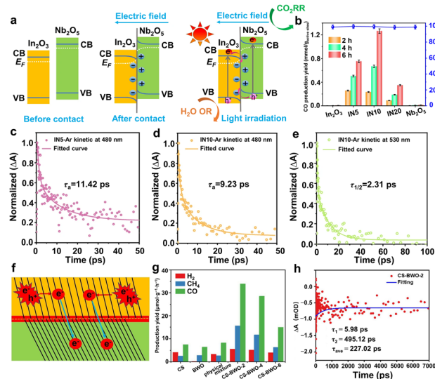
Fig. 4 (a) \text{In}_2\text{O}_3/\text{Nb}_2\text{O}_5 S-heterojunction formation and charge transfer mechanism. (b) The CO yield and selectivity of different catalysts. (c–e) Kinetic decay curves of the transient absorption spectra of different catalysts. Reproduced with permission from ref. 45. Copyright 2024, Springer Nature. (f) Scheme of a heterojunction with highly connected and matching crystal faces. (g) Product evolution rates of different catalysts. (h) Normalized transient absorption kinetics for \text{CuS-Bi}_2\text{WO}_6 . Reproduced with permission from ref. 46. Copyright 2024, Wiley-VCH.
