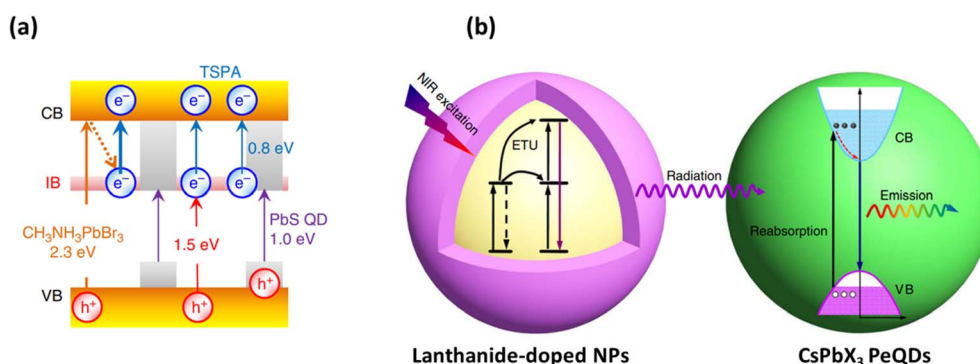
Fig. 2 (a) Schematic energy band diagram of the photo-absorption layer in an IB solar cell. EBG of MAPbBr 3 perovskite; 2.3 eV, EBG of PbS QD; 1.0 eV, EVI; 0.8 eV, EIC; 1.5 eV. Reproduced from Hosokawa et al. , Nat. Commun. , 2019, 19 © The Author(s), under exclusive licence to Springer Nature. Distributed under the terms of the Creative Commons Attribution 4.0 International License (CC BY 4.0) (b) schematic representation of the radiative energy transfer upconversion processes in all-inorganic CsPbX 3 perovskite quantum dots through sensitization by lanthanide-doped nanoparticle (the solid and dash lines represent the electronic transitions). 20 Adopted from Zheng et al. , Nat. Commun. , 2018, 20 © The Author(s), published by Springer Nature, under the terms of the Creative Commons Attribution 4.0 International License (CC BY 4.0).
