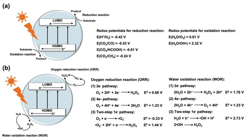
Fig. 3 Schematic illustration of the processes of photocatalytic water splitting, carbon dioxide reduction (a) and hydrogen peroxide production (b), and corresponding redox potentials of the relevant reactions.
