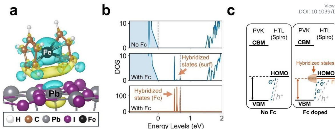
Figure 4. DFT modelling of the impact of residual ferrocene, the by-product of ferrocenium doping. a , Side view of the simulated lowest-energy configuration of ferrocene on the (001) \text{PbI}_2 -terminated \text{MAPbI}_3 surface and charge density profile (with charge density gain and loss coloured in yellow and blue, respectively). b , Calculated electronic density of states (DOS) for the \text{MAPbI}_3 surface with and without Fc doping. DOS are projected onto atoms in the top three layers of the surface slab (blue) and onto ferrocene atoms (orange). Top panel: surface without ferrocene; middle and bottom panels: surfaces with the ferrocene molecule relaxed near the surface, showing additional hybridized states not found in the undoped system. All DOS plots are aligned to the surface VBM, set to zero on the energy axis. The black dashed line indicates the position of the highest occupied level at the surface. c , Schematic energy level diagram illustrating the proposed mechanism of hole transport at the interface between the perovskite (PVK) layer and the HTL without (left) and with (right) Fc doping.
