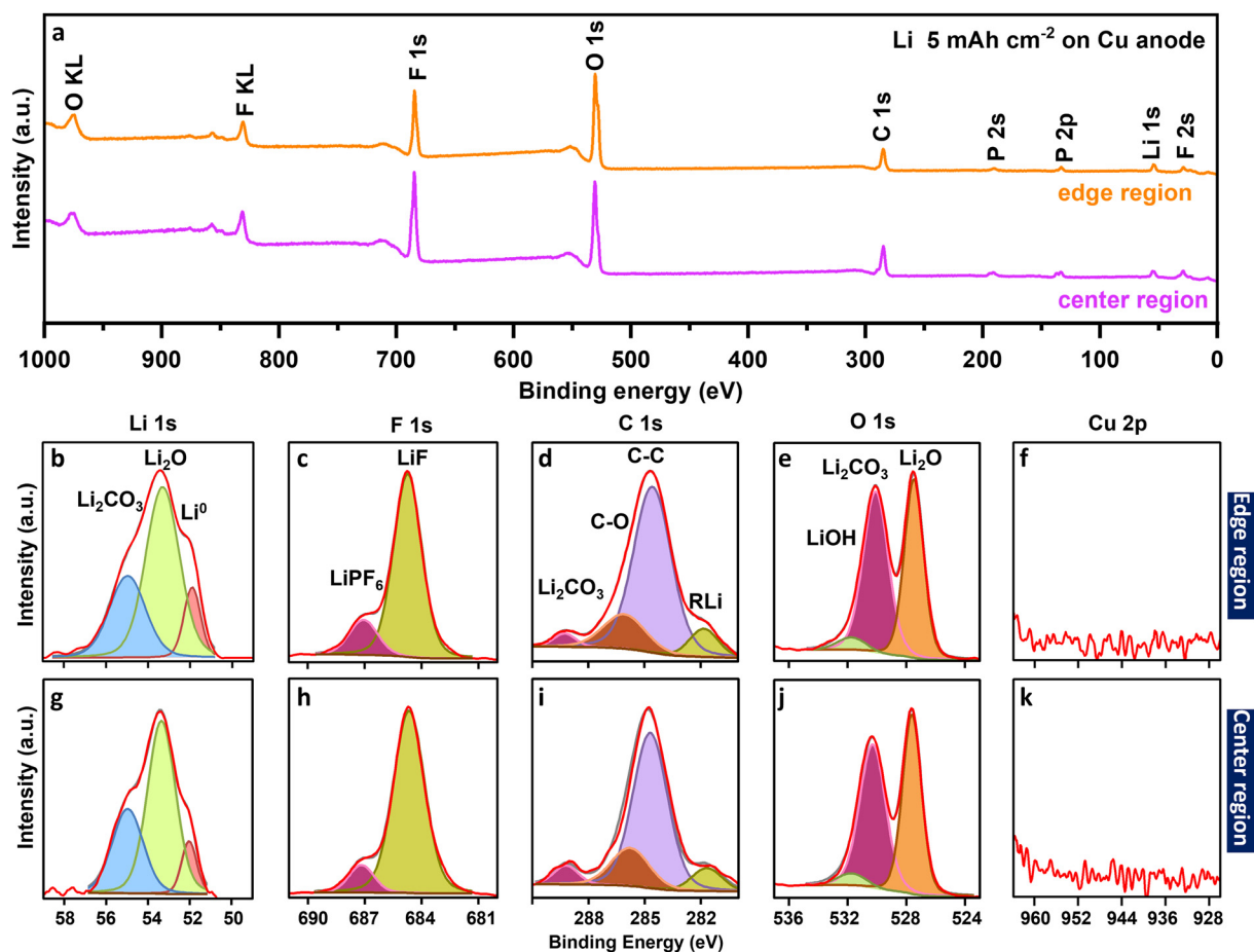
Fig. 8 (a) XPS survey spectra of the annular edge and center regions in plated lithium metal at a capacity of 5 \text{ mA h cm}^{-2} . High-resolution XPS spectra of the (b)–(f) annular edge and (g)–(k) center regions in 5 \text{ mA h cm}^{-2} plated lithium metal, showing Li 1s, F 1s, C 1s, O 1s, and Cu 2p excitation peaks.
