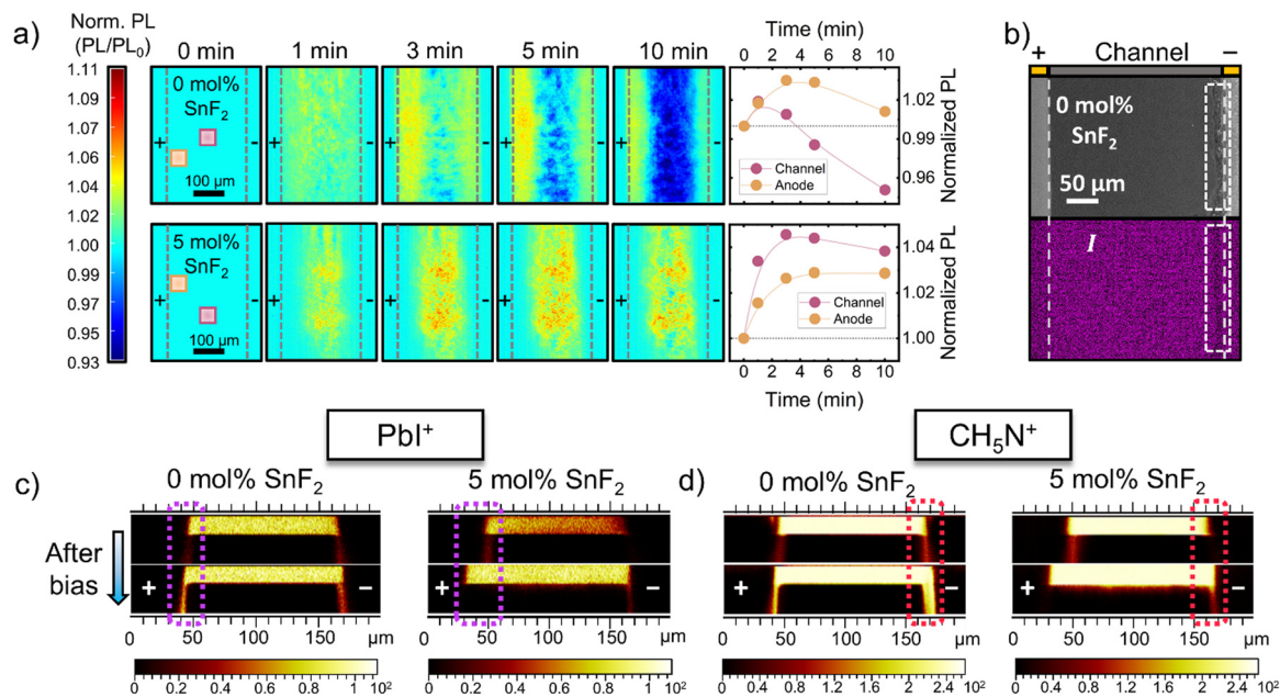
Fig. 5 (a) Hyperspectral PL maps from the Au/Cr/FASn 0.5 Pb 0.5 I 3 (channel length is 300 \mu\text{m} )/Cr/Au lateral devices upon 30 V bias, the SnF 2 concentrations are: 0 mol% and 5 mol%. We tracked the PL emission from mainly two areas: the channel and the anode, these are indicated by the pink and orange squares on the 0 min frames for each sample. Each frame was recorded every 1 minute. For clarity, we only displayed 5 frames per sample. The rest of the data set can be found in Fig. S10b (ESI † ). (b) SEM images (top panel) and I EDS elemental maps (bottom panel) from the 0 mol% sample after 30 V bias for 1 hour. The white square highlights the damaged region after biasing. ToF-SIMS x - z depth profile maps of: (c) PbI + and (d) CH 5 N + fragments from the 0 and 5 mol% SnF 2 samples before and after bias.
