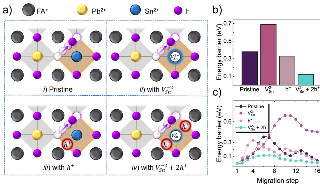
Fig. 4 (a) Theoretical model of the iodide migration pathway in a \text{FAPb}_{0.5}\text{Sn}_{0.5}\text{I}_3 lattice under four scenarios: (i) \text{V}_1^+ ( i.e. the pristine case), (ii) \text{V}_1^+ and \text{V}_{\text{Sn}}^{2-} , (iii) \text{V}_1^+ and \text{h}^+ , and (iv) \text{V}_1^+ , \text{V}_{\text{Sn}}^{2-} , and 2\text{h}^+ . (b) The energy barriers for iodide migration of each proposed scenario. (c) Relative energy landscapes of the system during iodide migration, the x-axis represents the iodide migration step during its transition towards an adjacent \text{V}_1^+ .
