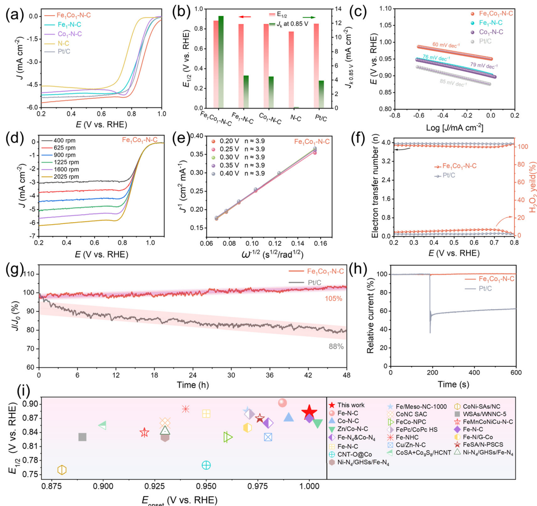
Fig. 4 Electrochemical ORR performance evaluated by RDE and RRDE tests. (a) LSV curves, (b) comparison of E_{1/2} and J_k at 0.85 V, and (c) Tafel plots for Fe 1 Co 1 -N-C and reference samples (Fe 1 -N-C, Co 1 -N-C, and Pt/C). (d) Polarization curves of Fe 1 Co 1 -N-C at different rotation rates and (e) the K-L fitting lines at different potentials. (f) \text{H}_2\text{O}_2 yield and the electron transfer number ( n ) values for Fe 1 Co 1 -N-C and Pt/C. (g) Normalized chronoamperometric curves of the ORR for Fe 1 Co 1 -N-C and Pt/C during 48 h stability tests. (h) Chronoamperometric methanol resistance tests of Fe 1 Co 1 -N-C and Pt/C. (i) Activity comparison of Fe 1 Co 1 -N-C with other reported ORR catalysts. The Fe 1 Co 1 -N-C exhibits a high ORR catalytic activity and excellent stability in the three-electrode system.
