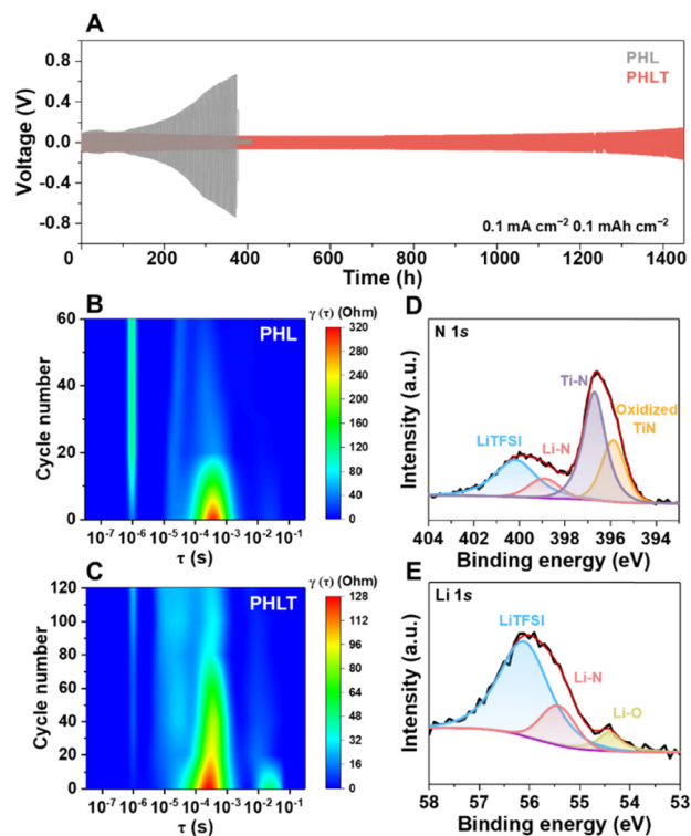
Fig. 4 (A) Lithium stripping-plating profiles at 0.1 mA cm -2 and 0.1 mA h cm -2 . DRT results of (B) Li|PHL|Li and (C) Li|PHLT|Li cells cycled at 0.2 mA cm -2 and 0.2 mA h cm -2 . Ex situ XPS analysis of (D) N 1s and (E) Li 1s spectra of recovered TiN nanofibers.
