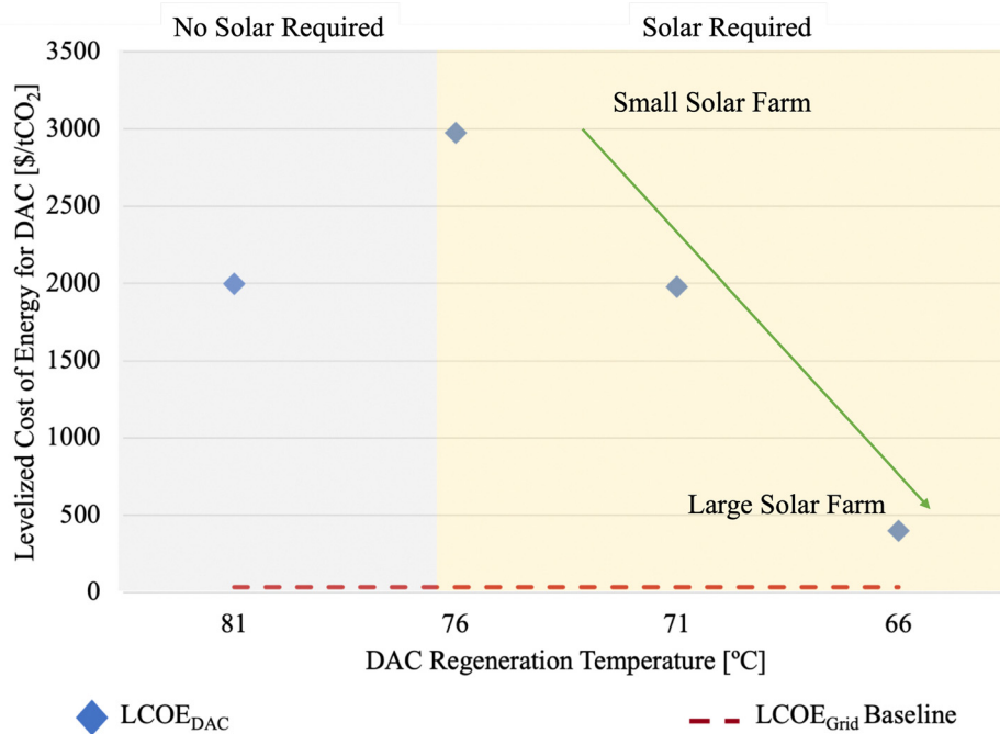
Fig. 8 Levelized cost of energy for DAC delivered by the DAC in series – upstream configuration using a low-temperature geothermal reservoir, compared to the baseline levelized cost of the grid electricity generation baseline case.
