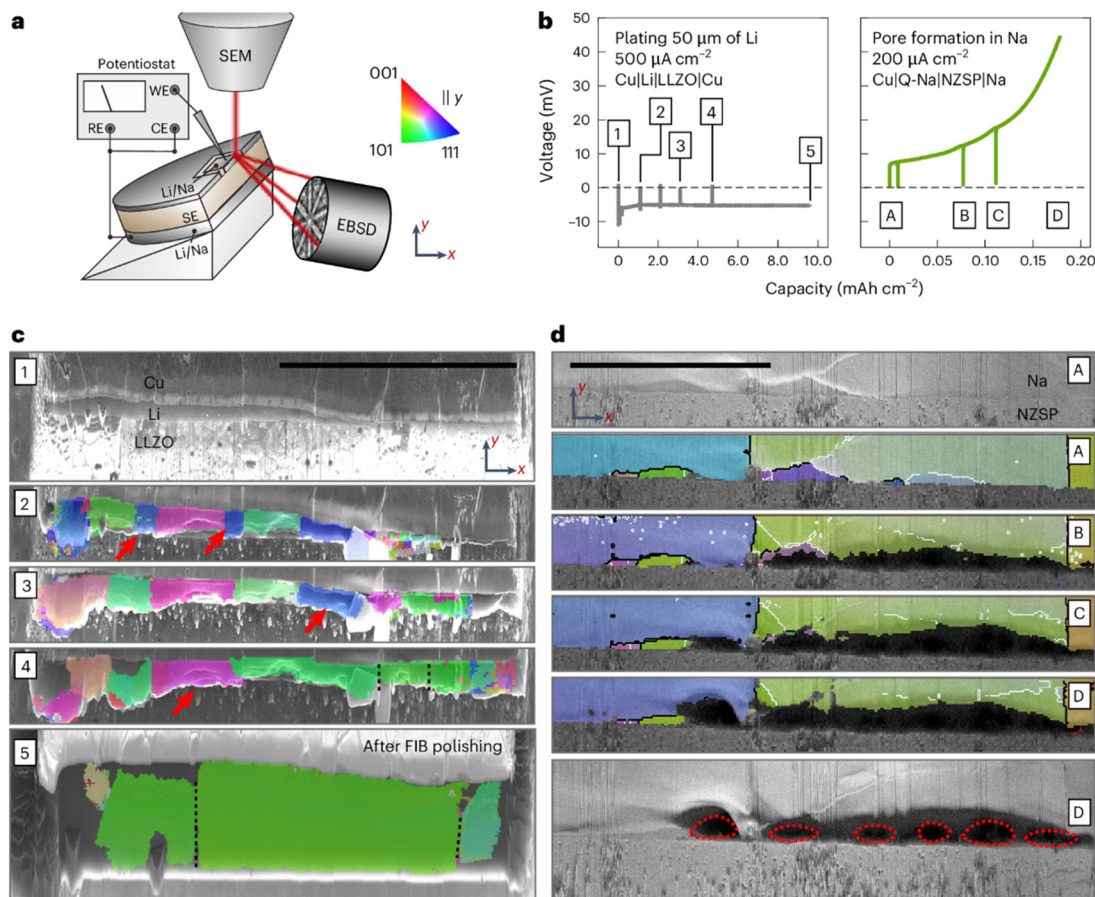
Fig. 28 In situ EBSD approach for examining the microstructural changes occurring during the electrodeposition and electrodedissolution of an alkali metal electrode in contact with a solid electrolyte. (a) A schematic representation of the in situ EBSD setup. (b) Voltage profiles for depositing 50 \mu\text{m} of Li at the Cu|Li|SE interface and for stripping Na until pore formation occurs at the Cu|Q-Na|SE interface. (c) Microstructural changes during Li plating. (1) shows an SEM image of the pristine cross-section of Cu|Li|SE. The lithium reservoir is not freshly deposited, and is also too thin to obtain EBSDs of sufficient quality to generate an IPF map. However, upon depositing around 10–15 \mu\text{m} of additional lithium, the IPF map depicted in (2) was obtained. Herein, several grains around 10–30 \mu\text{m} wide are visible. Surprisingly, after another \sim 5 \mu\text{m} of lithium deposition, fewer but wider grains are visible in the next IPF map in (3). Two small blue grains close to an <111> orientation from the previous map apparently fused into larger neighbouring grains close to an <101> orientation (green). After another deposition step, IPF map (4) shows even wider grains, with another blue grain from the previous map being fused to a neighbouring green grain. After another long deposition step resulting in around 20 \mu\text{m} of additional lithium, multiple grains have fused together forming a large grain with >100 \mu\text{m} width, again close to a <101> orientation as visible in (5). (d) Microstructural changes during Na stripping. Starting from an optimal interfacial contact between sodium and SE (A), a dark region close to the interface emerges (B) after the first stripping interval, attributed to pores. Interestingly, the pores formed mainly within the green grain, while the vertical grain boundaries on both sides remain intact (C). As stripping progresses, another pore nucleates within the large blue grain starting from a grain boundary, supporting the previous description. Moreover, the pores within the green grain further grow into its bulk (D). 349
