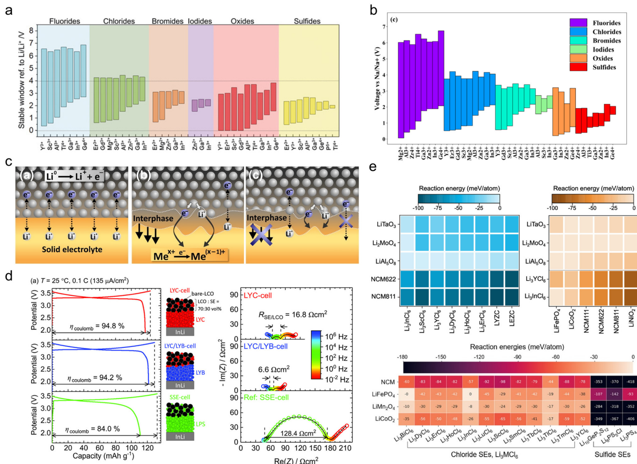
Fig. 7 The thermodynamic electrochemical windows of (a) \text{Li-M-X} ( X = \text{F, Cl, Br, I, O, S} ) 75 and (b) \text{Na-M-X} through calculation. 122 (c) Three types of interfaces between lithium metal and solid electrolytes. 124 (d) Initial charge/discharge curves and the impedance value of \text{Li}_3\text{YCl}_6 after the first charging cycling. 34 (e) The reaction energy calculations between different cathode materials and halide electrolytes based on various metal cations. 123,125
