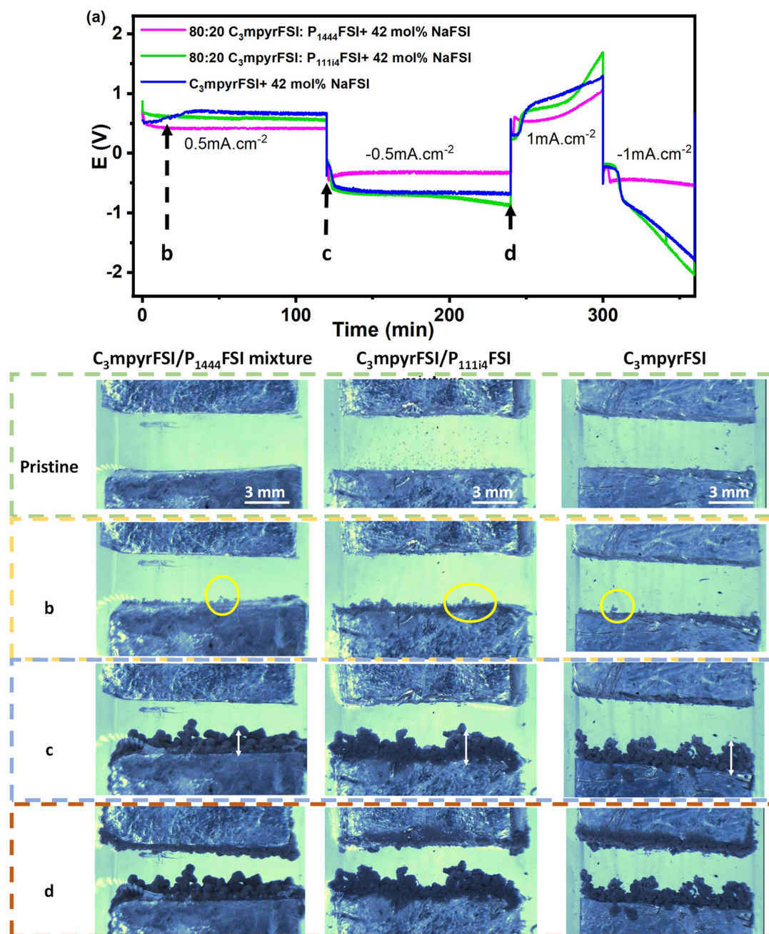
Fig. 8 In situ optical micrographs obtained for flooded optical cell cycled at 0.5 mA cm -2 . (a) Cycling profile and morphology are shown at pristine; (b) after 10 min (Na deposition); (c) after first half-cycle; (d) after first cycle.
