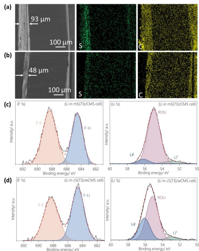
Figure 6. Lithium anode characterization of different S/CMS composites included cells. (a-b) SEM images and elemental mapping of lithium anode cross section. (a) mS(73)/CMS. (b) cS(73)/wCMS. (c-d) XPS spectra of lithium anode. (c) mS(73)/CMS. (d) cS(73)/wCMS.
