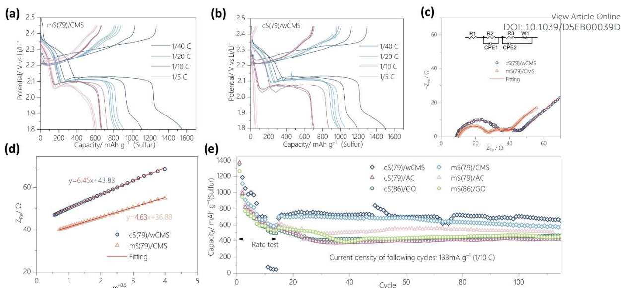
Figure 3. Electrochemical properties of S/CMS composites. (a,b) GCD curves of (a) mS(79)/CMS and (b) cS(79)/wCMS under different rates. (c) Nyquist plots after cell discharging to 2.15 V. (d) The relationship between real part of impedance and the inverse square root of angular frequency. (e) Cycling stability performance. The initial 14 cycles were conducted at varying rates, as shown in a and b. Starting from the 15 th cycle, a constant current density of 133 mA g -1 (1/10C) was applied. The electrolyte is 1 M LiTFSI + 1 M LiNO 3 + 0.08 M La(NO 3 ) 3 in DME/DOL.
