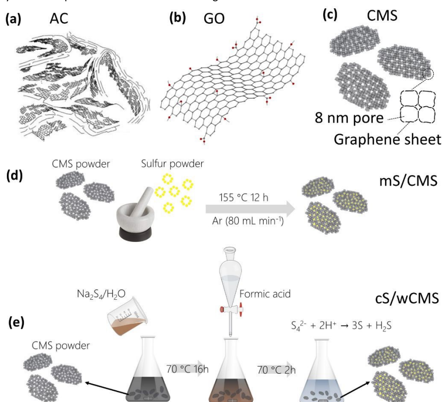
Figure 1. Carbon materials utilized in this study. (a) Activated carbon (AC). (b) Graphene oxide (GO). (c) Carbon mesosponge (CMS). (d,e) The preparation scheme of S-loaded samples. (d) Melt diffusion method. (e) Chemical reaction method.
