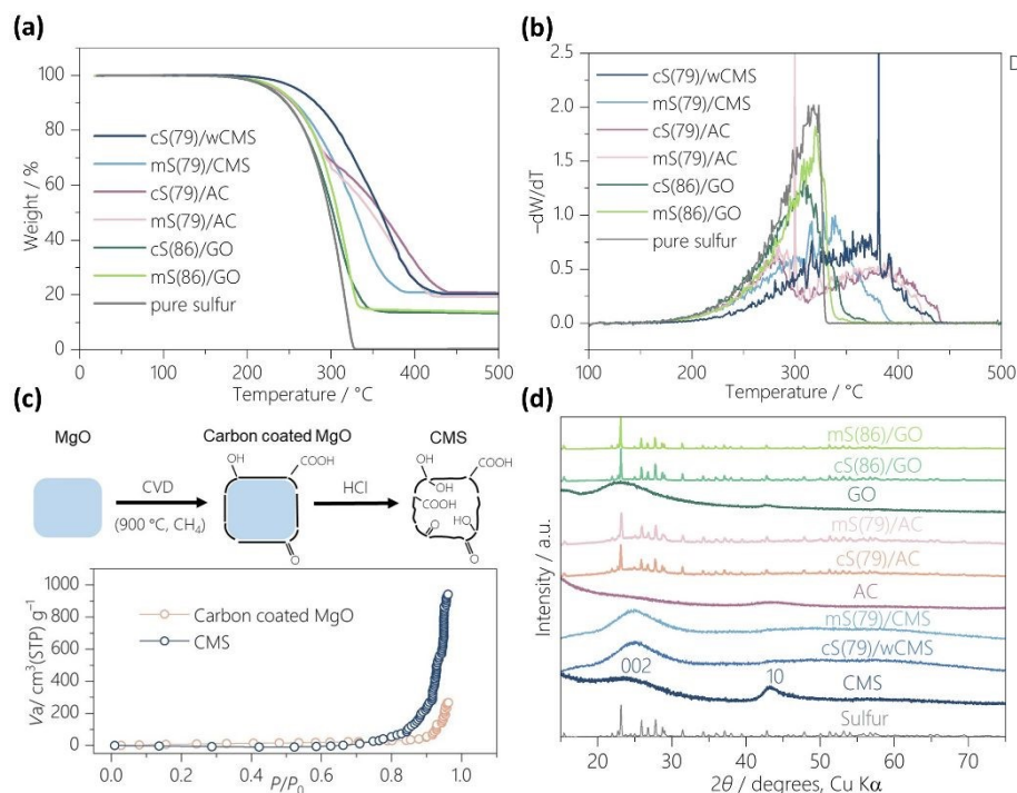
Figure 2. Analysis of sulfur loaded on carbon scaffolds. (a) TG curves of sulfur/carbon composites under nitrogen atmosphere. (b) Derivative weight loss versus temperature obtained from TGA results. (c) Preparation scheme of CMS (top) and water vapor adsorption isotherms of CMS before and after template removal (bottom). (d) XRD patterns.
