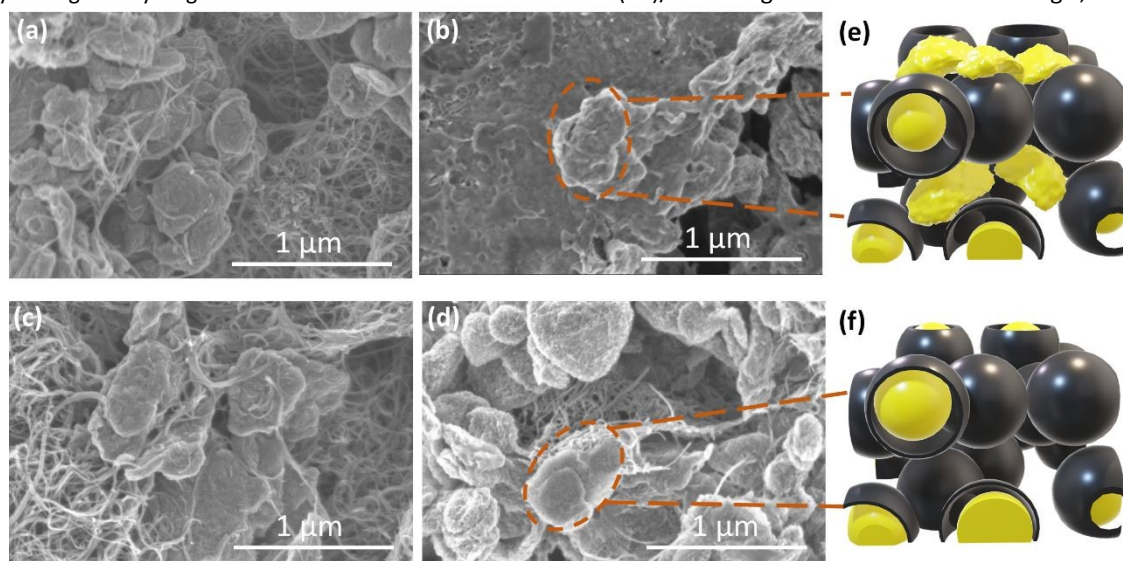
Figure 4. Electrode morphology of different S/CMS composites. (a,b) SEM images of mS(79)/CMS. (a) Pristine status. (b) After one cycle discharge-charge. (c,d) SEM images of cS(79)/wCMS. (c) Pristine status. (d) After one cycle discharge-charge. (e,f) Illustration showing sulfur and lithiated sulfur in (e) mS(79)/CMS and (f) cS(79)/wCMS.
