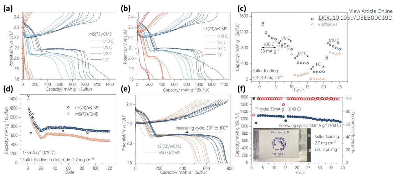
Figure 5. Electrochemical measurements of S/CMS composites with an optimized sulfur content (73 wt%). (a,b) GCD curves of (a) mS(73)/CMS and (b) cS(73)/wCMS under different rates. (c) Rate performance. (d) Cycling stability. (e) GCD curves during cycling tests. (f) Cycling test of a pouch cell using cS(73)/wCMS.
