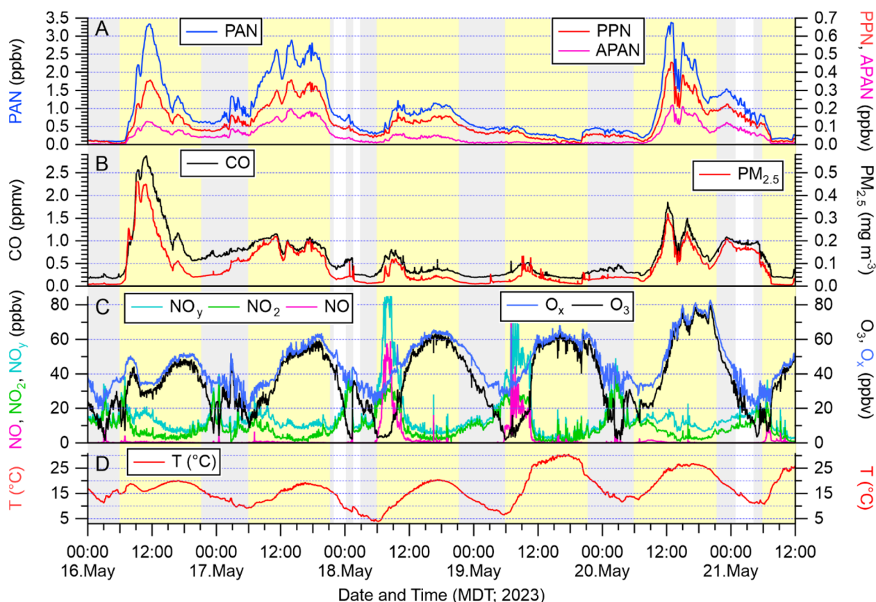
Fig. 5 Partial time series of quantities measured during FOOBAR. (A) PAN (left axis) and PPN and APAN (right axis). (B) Carbon monoxide (CO; left axis) and PM 2.5 (right axis). (C) Nitric oxide (NO), nitrogen dioxide (NO 2 ) and total odd nitrogen (NO y ; left axis), and ozone (O 3 ) and odd oxygen (O x = O 3 + NO 2 ; right axis). (D) Ambient air temperature. The background shading indicates night (light gray) and day (light yellow). Regions shaded in white colour were selected for further analysis (see text).
