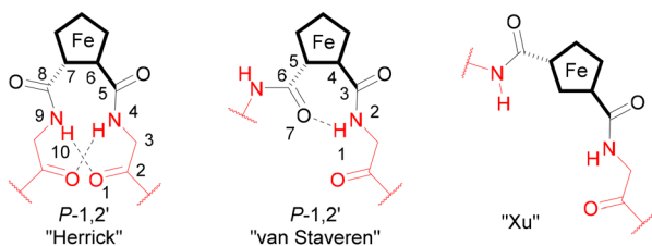
Fig. 2 Hydrogen bonding motifs in substituted 1,n' -ferrocenyl peptides. Bold lines represent bonds spatially in front of the rest of the molecule, and dashed lines represent bonds spatially behind the rest of the molecule.
