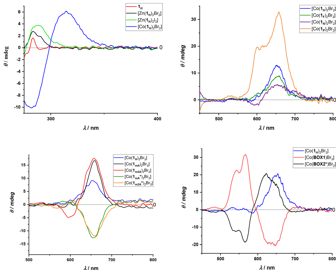
Fig. 8 Overlapped CD spectra in \text{CH}_2\text{Cl}_2 of: ligand 1 H and corresponding zinc(II) and cobalt(III) halide complexes at c = 0.075 mM (top left); cobalt(III) bromide complexes of ligands 1 H , 1 F , 1 N and 1 P in the visible region of the spectrum at c = 1.13 mM (top right); cobalt(III) bromide complexes of ligands 1 H , 1 mA , 1 mA * , 1 m2A and 1 m2A * in the visible region of the spectrum at c = 0.74 mM (bottom left); and cobalt(III) bromide complexes at c = 2.25 mM with ligands 1 H , (–)-2,2'-isopropylidenebis[(4 S )-4-phenyl-2-oxazoline] ( BOX1 ) and (+)-2,2'-isopropylidenebis[(4 R )-4-benzyl-2-oxazoline] ( BOX2* ) (bottom right).
