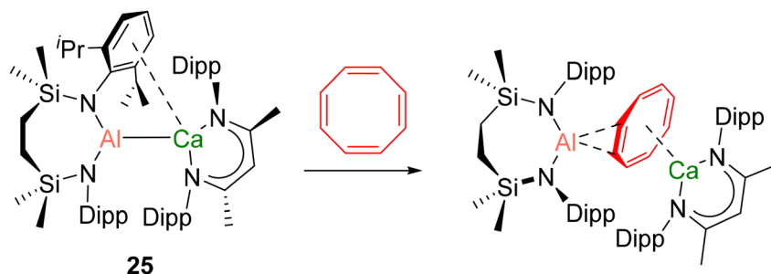
Scheme 11 Reaction of calcium alumanyl complex 23 with cyclooctatetraene.
