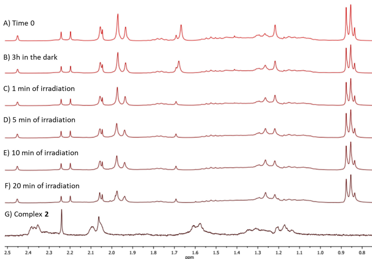
Fig. 5 ^1\text{H} NMR spectra (300 MHz) of complex 4 (0.013 M) with 0.25 eq. of TARF (A) at time 0 in \text{CD}_2\text{Cl}_2 ; (B) after 3 h in the dark in \text{CD}_2\text{Cl}_2 ; (C) after 1 min of irradiation at 456 nm in \text{CD}_2\text{Cl}_2 ; (D) after 5 min of irradiation at 456 nm in \text{CD}_2\text{Cl}_2 ; (E) after 10 min of irradiation at 456 nm in \text{CD}_2\text{Cl}_2 ; (F) after 20 min of irradiation at 456 nm in \text{CD}_2\text{Cl}_2 . Finally, (G) is the ^1\text{H} NMR spectrum (300 MHz) of the derived complex 2 in \text{D}_2\text{O} .
