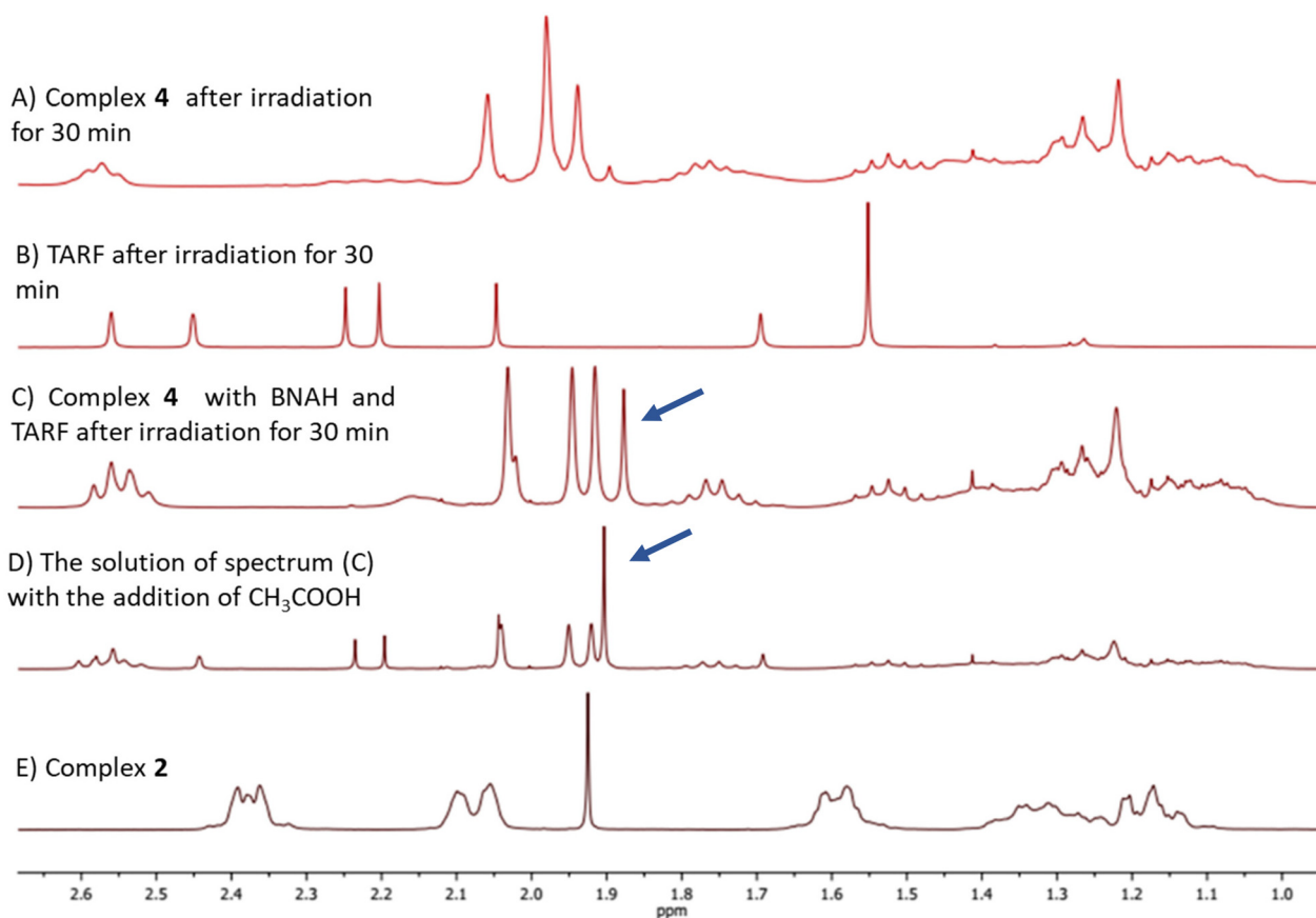
Fig. 2 ^1\text{H} NMR spectra (300 MHz) of (A) complex 4 (0.013 M) after irradiation for 30 min at 365 nm in \text{CD}_2\text{Cl}_2 ; (B) TARF (0.003 M) after irradiation for 30 min at 365 nm in \text{CD}_2\text{Cl}_2 ; (C) complex 4 (0.013 M) with 4.00 eq. of BNAH and 0.25 eq. of TARF after irradiation for 30 min at 365 nm in \text{CD}_2\text{Cl}_2 ; (D) the solution of spectrum (C) after the addition of 1 \mu\text{L} of \text{CH}_3\text{COOH} and 49 \mu\text{L} of \text{CD}_2\text{Cl}_2 ; (E) complex 2 – precipitated from the solution of spectrum (C) – in \text{D}_2\text{O} . Peaks corresponding to \text{CH}_3\text{COOH} in spectra (C) and (D) are highlighted with blue arrows.
