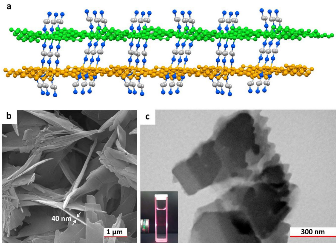
Fig. 4 (a) Suggested multilayer structure of Zn-CP-en as the second PSM product. (b and c) FE-SEM and TEM images of Zn-CP-en (inset in c: the Tyndall effect of an ethanolic colloidal suspension of Zn-CP-en ).
