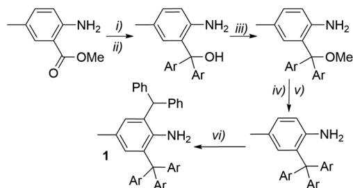
Scheme 4 The synthesis of \text{Ar}^{\text{t-Bu}}\text{-NH}_2 ( 1 ). (i) 4- t -Bu- \text{C}_6\text{H}_4\text{MgBr} ; (ii) \text{NH}_4\text{Cl} ; (iii) \text{CH(OMe)}_3/\text{H}_2\text{SO}_4 ; (iv) 4- t -Bu- \text{C}_6\text{H}_4\text{MgBr} ; (v) \text{NH}_4\text{Cl} ; and (vi) \text{Ph}_2\text{CH(OH)/ZnCl}_2/\text{HCl} .
