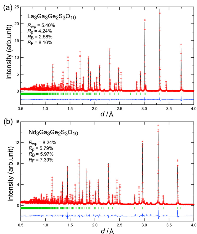
Fig. 5 Neutron powder diffraction patterns collected from (a) \text{La}_3\text{Ga}_3\text{Ge}_2\text{S}_3\text{O}_{10} and (b) \text{Nd}_3\text{Ga}_3\text{Ge}_2\text{S}_3\text{O}_{10} at room temperature. Rietveld refinements were performed on the basis of the structural models determined by single crystal structure analysis.
