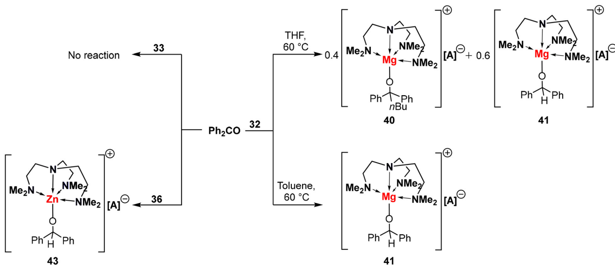
Scheme 10 Reactivity of the n -butylmagnesium cation 32 and the hydrido-zinc cation 36 towards electrophiles like \text{CO}_2 (top) and \text{Ph}_2\text{CO} (bottom).
