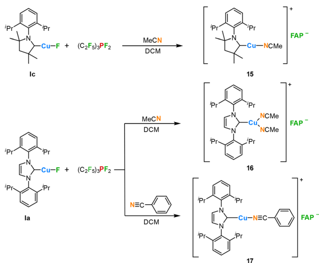
Scheme 3 Synthesis of [(\text{carbene})\text{Cu}(\text{LB})]^+\text{FAP}^- complexes 15–17 via fluoride ion abstraction from [(\text{carbene})\text{CuF}] using (\text{C}_2\text{F}_5)_3\text{PF}_2 in the presence of N-donor ligands.
