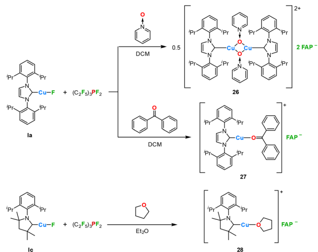
Scheme 6 Synthesis of complexes 26–28 via fluoride ion abstraction from [(carbene)CuF] using (C 2 F 5 ) 3 PF 2 in the presence of O-donor ligands.
