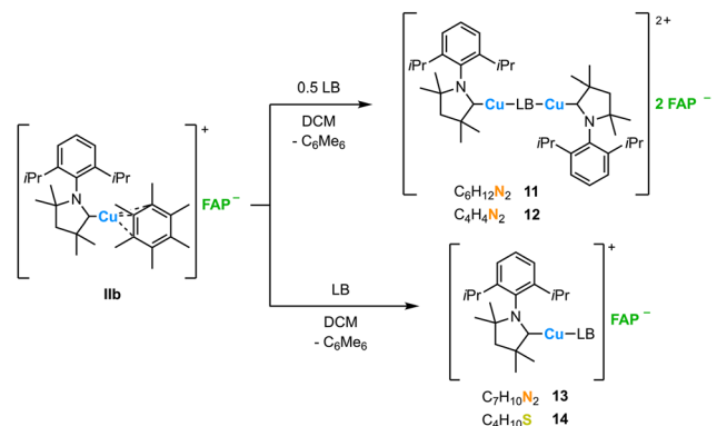
Scheme 2 Synthesis of [(\text{cAAC}^{\text{Me}})\text{Cu}]_2(\text{C}_6\text{H}_{12}\text{N}_2)]^{2+} 2\text{FAP}^- ( 11 ), [(\text{cAAC}^{\text{Me}})\text{Cu}]_2(\text{C}_4\text{H}_4\text{N}_2)]^{2+} 2\text{FAP}^- ( 12 ), [(\text{cAAC}^{\text{Me}})\text{Cu}(\text{C}_7\text{H}_{10}\text{N}_2)]^+\text{FAP}^- ( 13 ), and [(\text{cAAC}^{\text{Me}})\text{Cu}(\text{C}_4\text{H}_{10}\text{S})]^+\text{FAP}^- ( 14 ) via hexamethylbenzene substitution of [(\text{cAAC}^{\text{Me}})\text{Cu}(\text{C}_6\text{Me}_6)]^+\text{FAP}^- ( IIb ).
