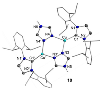
Fig. 2 Molecular structure of the complex cation of [(\text{IDipp})\text{Cu}]_2(\text{C}_2\text{N}_3\text{H}_3)_2]^{2+} 2\text{FAP}^- ( 10 ) in the solid state (ellipsoids set at the 50% probability level; Dipp substituents are shown as wire-and-stick models). Hydrogen atoms except for the ones bound to N5 and N6 and a co-crystallized solvent molecule are omitted for clarity. Selected bond length and angles are collected in Table 2 and Fig. S6 in the ESI.†
