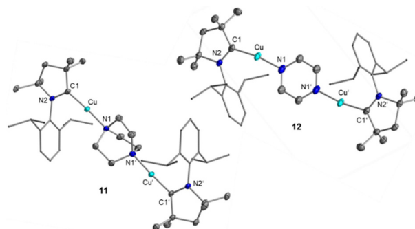
Fig. 3 Molecular structures of the complex cations of [(\text{cAAC}^{\text{Me}})\text{Cu}]_2(\text{C}_6\text{H}_{12}\text{N}_2)]^{2+} 2\text{FAP}^- ( 11 ; left) and [(\text{cAAC}^{\text{Me}})\text{Cu}]_2(\text{C}_4\text{H}_4\text{N}_2)]^{2+} 2\text{FAP}^- ( 12 ; right) in the solid state (ellipsoids set at the 50% probability level; Dipp ligands are shown as wire-and-stick models). Hydrogen atoms are omitted for clarity. Selected bond length and angles are collected in Table 2 and Fig. S7, S8 in the ESI.†
