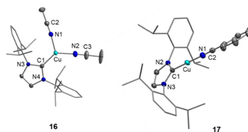
Fig. 4 Molecular structures of the complex cations of [(\text{IDipp})\text{Cu}(\text{N}\equiv\text{CMe})_2]^+\text{FAP}^- ( 16 ; left) and [(\text{IDipp})\text{Cu}(\text{N}\equiv\text{CPh})]^+\text{FAP}^- ( 17 ; right) in the solid state (ellipsoids set at the 50% probability level; Dipp substituents are shown as wire-and-stick models). Hydrogen atoms are omitted for clarity. Selected bond lengths and angles are collected in Table 3 and Fig. S9, S10 in the ESI.†
