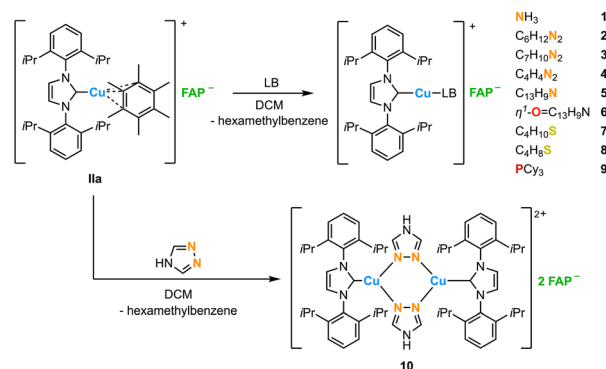
Scheme 1 Synthesis of [(\text{IDipp})\text{Cu}(\text{LB})]^+\text{FAP}^- (LB = \text{NH}_3 , 1 ; \text{C}_6\text{H}_{12}\text{N}_2 = DABCO, 2 ; \text{C}_7\text{H}_{10}\text{N}_2 = DMAP, 3 ; \text{C}_4\text{H}_4\text{N}_2 = pyrazine, 4 ; \text{C}_{13}\text{H}_9\text{N} = acridine, 5 ; \eta^1\text{-O}=\text{C}_{13}\text{H}_9\text{N} = acridone, 6 ; \text{C}_4\text{H}_{10}\text{S} = \text{SEt}_2 , 7 ; \text{C}_4\text{H}_8\text{S} = THT, 8 ; \text{PCy}_3 , 9 ) (top) and \{[(\text{IDipp})\text{Cu}]_2(\text{C}_2\text{N}_3\text{H}_3)_2\}^{2+}2\text{FAP}^- ( 10 , bottom, \text{C}_2\text{N}_3\text{H}_3 = 1,2,4, triazole) via substitution of hexamethylbenzene of [(\text{IDipp})\text{Cu}(\text{C}_6\text{Me}_6)]^+\text{FAP}^- ( IIa ).
