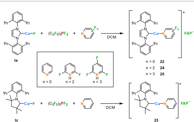
Scheme 5 Synthesis of [(carbene)Cu(LB)] + FAP − complexes 22–25 via fluoride ion abstraction from [(carbene)CuF] using (C 2 F 5 ) 3 PF 2 in the presence of (partially fluorinated) pyridine.
