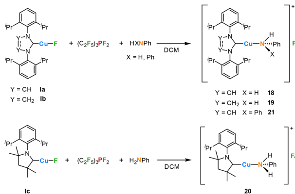
Scheme 4 Synthesis of [(carbene)Cu(LB)] + FAP − complexes 18–20 via fluoride ion abstraction from [(carbene)CuF] using (C 2 F 5 ) 3 PF 2 in the presence of amines.
