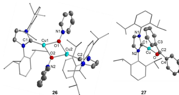
Fig. 7 Molecular structures of the complex cations of [(IDipp)Cu(μ-ONC 5 H 5 ) 2 ] 2+ 2FAP − ( 26 ; left) and [(IDipp)Cu(η 1 -O=CPh 2 )] + FAP − ( 27 ; right) in the solid state (ellipsoids set at the 50% probability level; Dipp substituents are shown as wire-and-stick models). Hydrogen atoms and two co-crystallized solvent molecules in the crystal structure of 26 are omitted for clarity. Selected bond lengths and angles are collected in Table 3 and Fig. S16, S17 in the ESI.†
