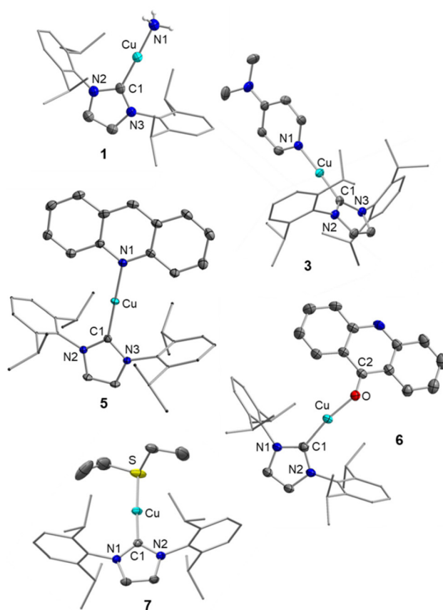
Fig. 1 Molecular structures of the complex cations of [(IDipp)Cu(NH 3 )] + FAP − ( 1 , top left), [(IDipp)Cu(C 7 H 10 N 2 )] + FAP − ( 3 , top right), [(IDipp)Cu(C 13 H 9 N)] + FAP − ( 5 , middle left), [(IDipp)Cu(η 1 -O=C 13 H 9 N)] + FAP − ( 6 , middle right) and [(IDipp)Cu(C 4 H 10 S)] + FAP − ( 7 , bottom) in the solid state (ellipsoids set at the 50% probability level; Dipp substituents are shown as wire-and-stick models). Hydrogen atoms (except the ones of NH 3 in 1 ) and co-crystallized solvent molecules in the crystal structures of 1 , 3 , and 6 are omitted for clarity. Only one of two independent molecules in the asymmetric unit of 1 and 3 are shown. Selected bond length and angles are given in Table 2 and Fig. S1–S5 in the ESI † .
