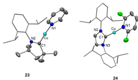
Fig. 6 Molecular structures of the complex cations of [(cAAC Me )Cu(NC 5 H 5 )] + FAP − ( 23 ; left) and [(IDipp)Cu(NC 5 H 5 )] + FAP − ( 24 ; right) in the solid state (ellipsoids set at the 50% probability level; Dipp substituents are shown as wire-and-stick models). Hydrogen atoms are omitted for clarity. Selected bond lengths and angles are collected in Table 3 and Fig. S14, S15 in the ESI.†
