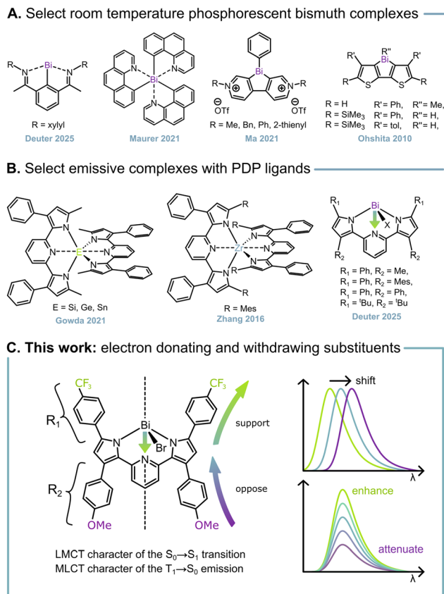
Fig. 1 (A) Compilation of the structures of select phosphorescent bismuth complexes that emit at r.t. in solution. 1–4 (B) Select main group element and Zr complexes with ligands containing the pyridine dipyrroliide structural motif. 5–7 (C) Concept for the design of the bismuth complexes reported in this manuscript.
