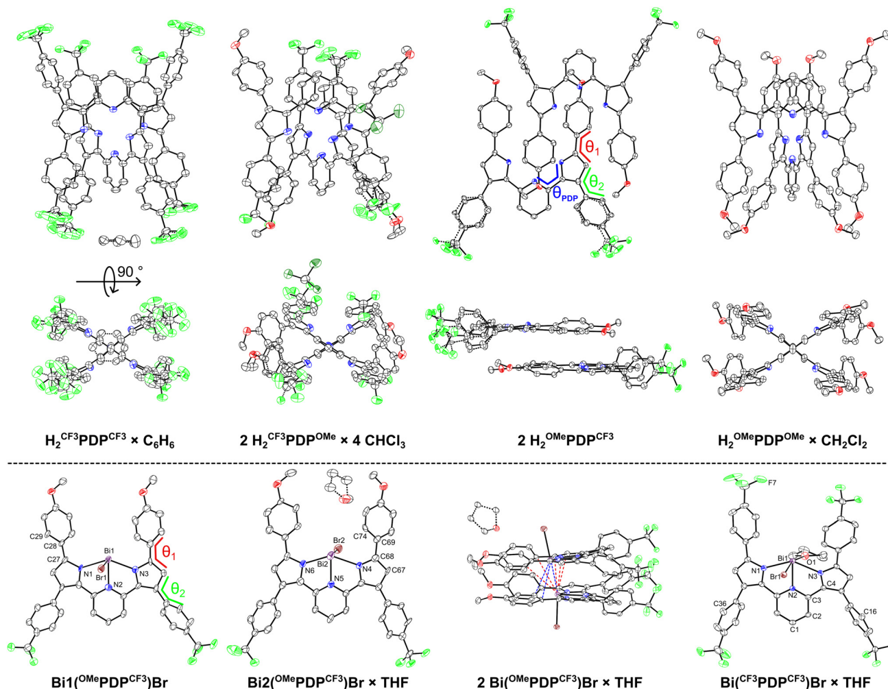
Fig. 6 Top: ORTEPs obtained for the solid-state structures of proligands \text{H}_2^{\text{R}1}\text{PDP}^{\text{R}2} . Thermal displacement ellipsoids are at the 50% probability level, with the exception of \text{H}_2^{\text{CF}_3}\text{PDP}^{\text{CF}_3} \times \text{C}_6\text{H}_6 , which is set at 30% for clarity. Angles discussed in the text are highlighted using one molecule within the asymmetric unit of \text{H}_2^{\text{OMe}}\text{PDP}^{\text{CF}_3} as an example. The co-crystallized \text{CH}_2\text{Cl}_2 solvent molecule within the solid-state structure of \text{H}_2^{\text{OMe}}\text{PDP}^{\text{OMe}} \times \text{CH}_2\text{Cl}_2 has been omitted for clarity reasons. Bottom: ORTEPs obtained for the solid-state structures of the two independent complex molecules of \text{Bi}(\text{OMePDP}^{\text{CF}_3})\text{Br} present within the unit cell and ORTEPs for the solid-state structure of \text{Bi}(\text{CF}_3\text{PDP}^{\text{CF}_3})\text{Br} . Thermal displacement ellipsoids are displayed at the 50% probability level. Angles discussed in the text are highlighted using one molecule within the asymmetric unit of 2 \text{Bi}(\text{OMePDP}^{\text{CF}_3})\text{Br} \times \text{THF} as an example.
