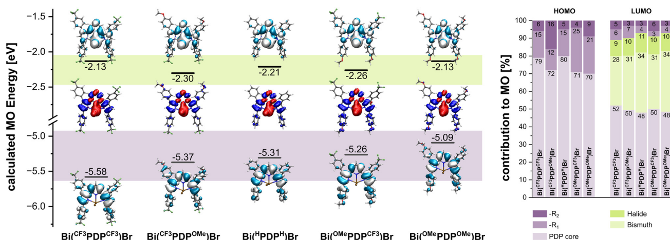
Fig. 4 Left: energy levels of the HOMO (purple shaded area) and the LUMO (green shaded area) of the complexes \text{Bi}(\text{R}^1\text{PDP}^{\text{R}2})\text{Br} , as well as depictions of the respective MOs in light blue and white and the corresponding electron density difference maps corresponding to the underlying HOMO–LUMO transition, with electron density loss in blue and electron density gain in red. Right: contributions of various fragments of the complexes \text{Bi}(\text{R}^1\text{PDP}^{\text{R}2})\text{Br} to the HOMO and LUMO as determined by TD-DFT calculations. \text{R}_1 and \text{R}_2 denote the contributions of the phenyl rings carrying the respective substituent.
