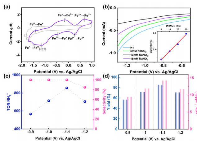
Fig. 4 (a) Cyclic voltammograms of H1 and ligand L in DMSO solution. (b) Linear sweep voltammograms of H1 (0.1 mM) with 0.1 M LiCl in DMSO/MOPS (v/v = 2 : 1) solution were recorded with the addition of \text{NO}_2^- . Inset: current intensity ( -1.1\text{ V} ) versus the concentration of \text{NO}_2^- . (c) The TON and selectivity of \text{NH}_4^+ under standard conditions. (d) Yield and rate of \text{NH}_4^+ produced by electrocatalytic \text{NO}_2^- reduction over the H1 catalyst.
