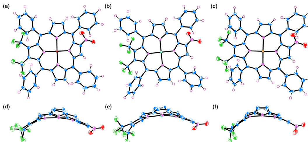
Fig. 1 ORTEP diagrams showing top (upper) and side views (lower) of CoTPP(NO 2 )(CF 3 ) 2 (a and d), NiTPP(NO 2 )(CF 3 ) 2 (b and e) and CuTPP(NO 2 )(CF 3 ) 2 (c and f). Solvates are omitted for clarity, and the meso -phenyls are removed for clarity in the side views (d–f). Color codes: C (slate blue), N (orchid), O (red), H (violet-red), F (lime green), Co (brown), Ni (orange), and Cu (cool copper).
