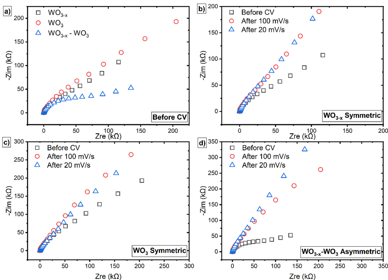
Fig. 10 Nyquist plots from impedance spectroscopy of \text{WO}_{3-x} and \text{WO}_3 nanowires in symmetric and asymmetric configurations. (a) Before CV analysis, (b) \text{WO}_{3-x} symmetric configuration, (c) \text{WO}_3 symmetric configuration, and (d) \text{WO}_{3-x}/\text{WO}_3 asymmetric configuration. The plots illustrate the impedance behavior before CV and after CV at 100 \text{ mV s}^{-1} and 20 \text{ mV s}^{-1} , highlighting the changes in charge transfer resistance and capacitance.
