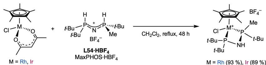
Scheme 21 Reaction of (S_P) -MaxPHOS (L54) with [M(\text{acac})\text{ClCp}^*] .
