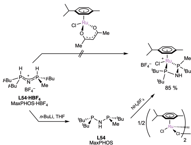
Scheme 22 Preparation of [\text{RuCl}(\text{L54})(p\text{-cymene})] .
