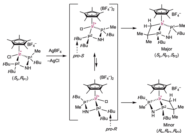
Scheme 23 C-H activation of t\text{-butyl} group on an iridium-L54 complex.
