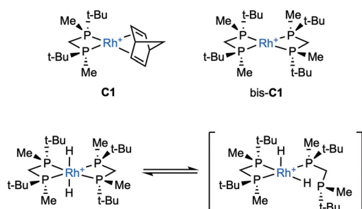
Fig. 4 Monochelated complex (C1) bischelated complex (bis-C1) (top). Equilibrium between the observed dihydrido species and the proposed hemilabile intermediate (bottom). Counter anions (PF 6 − or BF 4 − ) have been omitted for clarity.
