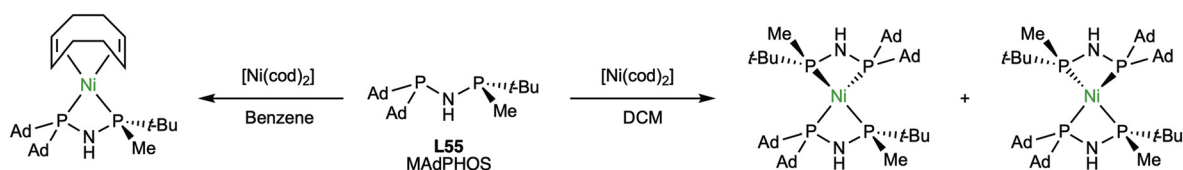
Scheme 20 Preparation of Ni(0)-MADPHOS (L55) complexes.
