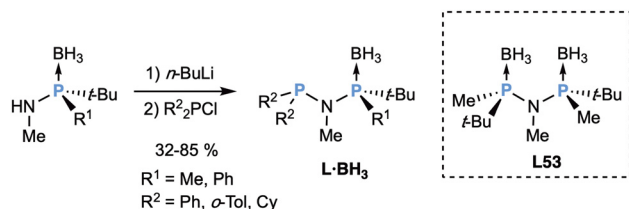
Scheme 13 Preparation of N -methyl substituted diphosphazane-boranes ( L\text{-BH}_3 ).
