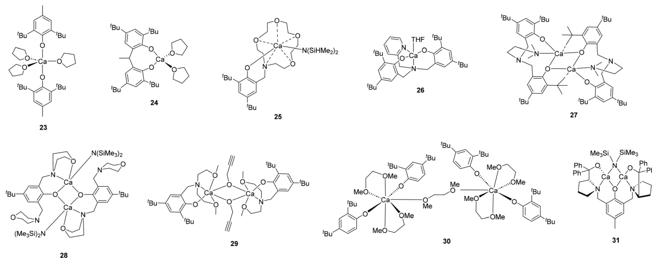
Fig. 3 Calcium catalysts supported by phenolate-based ligands for the ROP of cyclic esters.
