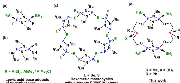
Fig. 1 (a and b) Selected examples of cyclodiphosphazane [\text{P}(\mu\text{-N}^t\text{Bu})_2]_2 -based adducts with main group Lewis acids; (c) an example of the heteroleptic \text{P}^{\text{V}}/\text{P}^{\text{III}} macrocycle; and (d) the newly synthesized first main group Lewis acid base adduct with phosphazane macrocycles.
