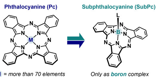
Fig. 1 Molecular structure of metalated Pcs and boron–SubPcs.
