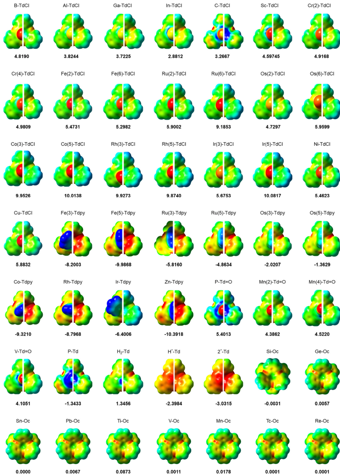
Fig. 5 DFT ESP maps of M-TdCl, M-TdpY, M-Oc, M-Td=O and M-Td complexes. Red color corresponds to a charge of -3.7 \times 10^{-2} , for neutral complexes, 0.075 for cationic complexes, -0.15 for H_1^- -Td, -0.25 for 2^- -Td; and the blue colour corresponds to a charge of 3.7 \times 10^{-2} , for neutral complexes, 0.11 for cationic complexes, 0.10 for H_1^- -Td, 0 for 2^- -Td.
