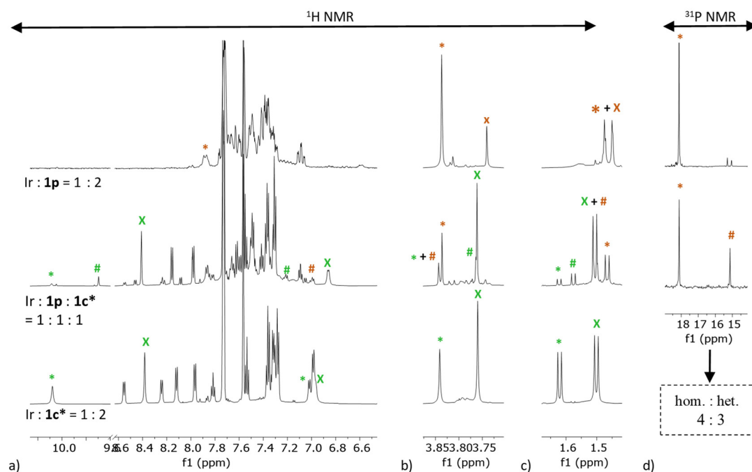
Fig. 5 Stacked 1 H NMR spectra (CD 2 Cl 2 ) of homoleptic and heteroleptic solutions of [Ir(COD) 2 ]BARF precursor and 1p ligand (orange) or/and 1c* ligand (green): (a) aromatic region, (b) functional group region, (c) aliphatic region. (d) Stacked 31 P NMR spectra. The homoleptic peaks are indicated by an asterisk (*), the heteroleptic peaks are indicated by a hash sign (#), the free ligand peaks are indicated by the letter (X). Abbreviations: hom.-homoleptic species; het.-heteroleptic species.
