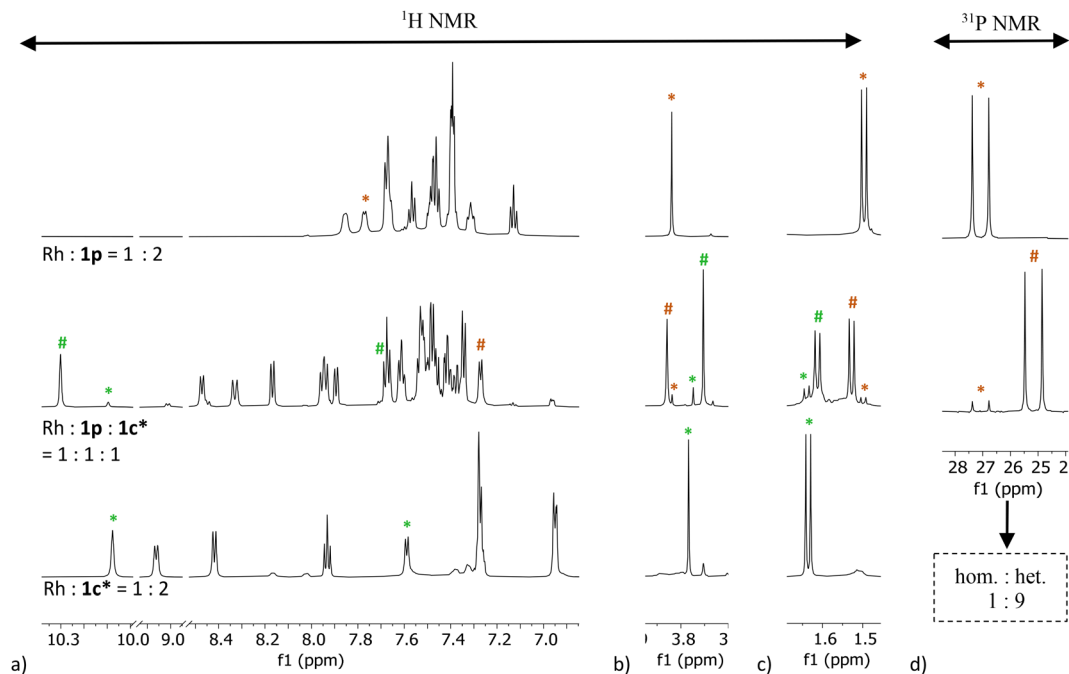
Fig. 4 Stacked 1 H NMR spectra (CD 2 Cl 2 ) of homoleptic and heteroleptic solutions of [Rh(COD) 2 ]BF 4 precursor and 1p ligand (orange) or/and 1c* ligand (green): (a) aromatic region, (b) functional group region, (c) aliphatic region. (d) Stacked 31 P NMR spectra. The homoleptic peaks are indicated by an asterisk (*) and the heteroleptic peaks are indicated by a hash sign (#). Abbreviations: hom.-homoleptic species; het.-heteroleptic species.
