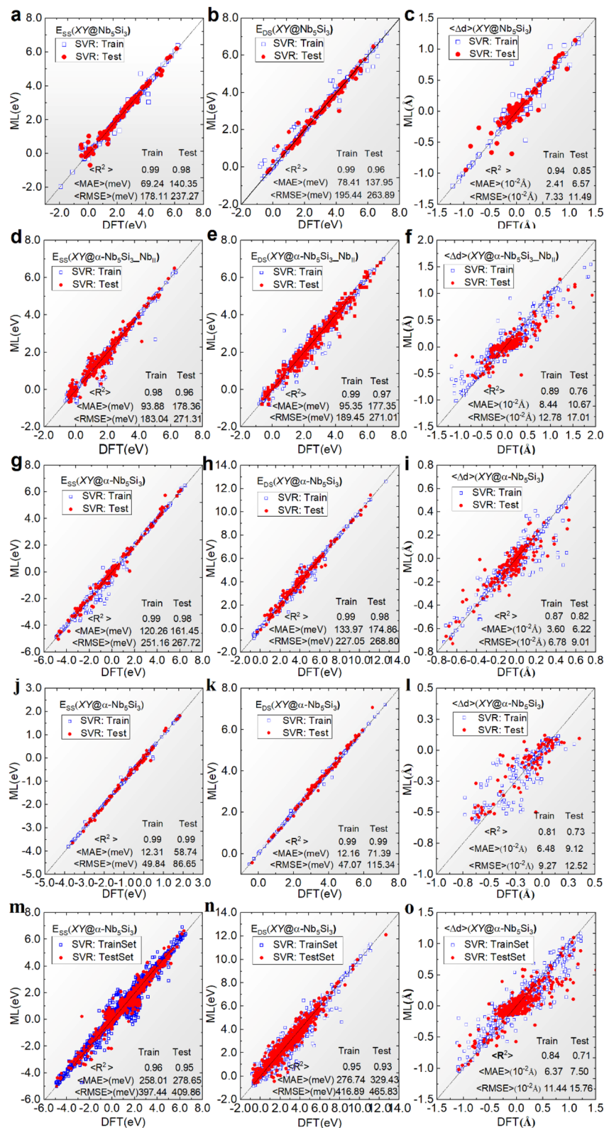
Fig. 4 E_{SS} , E_{DS} , and \langle \Delta d \rangle of the \alpha - Nb_5Si_3 substitution systems at the four non-equivalent sites (a–c) Nb_I , (d–f) Nb_{II} , (g–i) Si_I , (j–l) Si_{II} , and (m–o) all sites predicted by the CE AET -SVR models compared with the DFT results.
