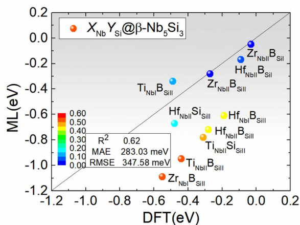
Fig. 9 Double-site substitution energies ( E_{DS} ) of the stable double-site substitution systems X_{Nb}Y_{Si}@-\beta-Nb_5Si_3 predicted by the ML models (CE AET -SVR) and DFT. The colored scale bar indicates the absolute errors from low (in blue) to high (in red).
