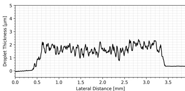
(a) \text{FAPbI}_3\text{-MAPbI}_3 Droplet Thickness Profile
