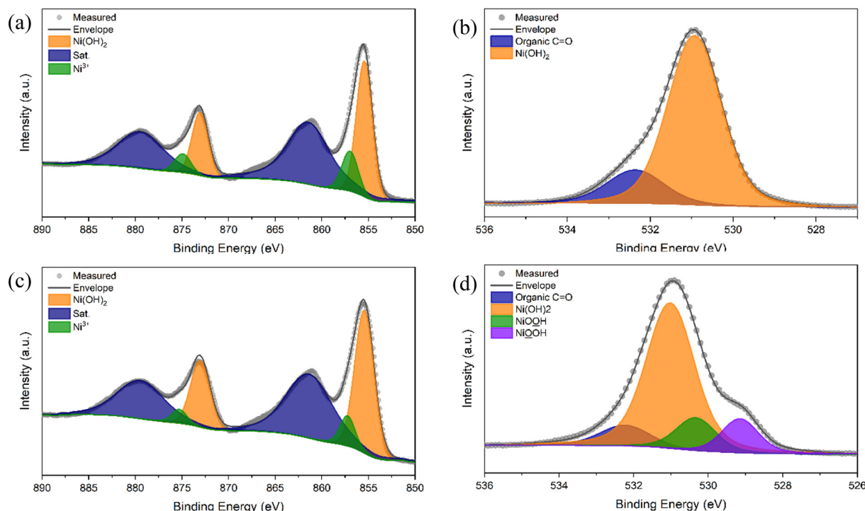
Fig. 5 XPS spectra of the fitted (a) Ni 2p and (b) O 1s regions of the electrodeposited \text{Ni}(\text{OH})_2 coating and the corresponding (c) Ni 2p and (d) O 1s regions of the electrochemically oxidised \text{NiOOH} sample, including the deconvoluted components. The \text{NiOOH} sample was prepared by anodic oxidation of the \text{Ni}(\text{OH})_2 coating at 1.49 V vs. RHE for 1 minute.
