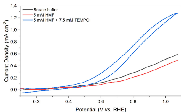
Fig. 3 Photocurrents of BiVO 4 photoanodes. LSV and CV with electrolyte with and without 5 mM HMF and 7.5 mM TEMPO. Scan rate = 10 mV s −1 .
