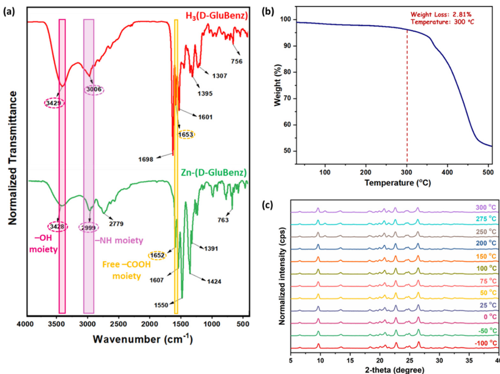
Fig. 1 (a) Comparison of FTIR spectra of H_3(D\text{-GluBenz}) and Zn-(D\text{-GluBenz}) , highlighting the catalytic sites, (b) thermogravimetric analysis profile and (c) VT PXRD patterns from -100 to +300 °C of Zn-(D\text{-GluBenz}) .
